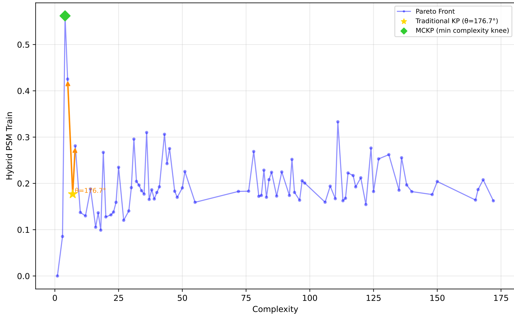
542_pollution - Run 24 - MVP - Hybrid PSM Train \lambda_1=1.00, \lambda_2=0.10, \lambda_3=0.00 | Difficulty: 0.39 | Method: mckp
