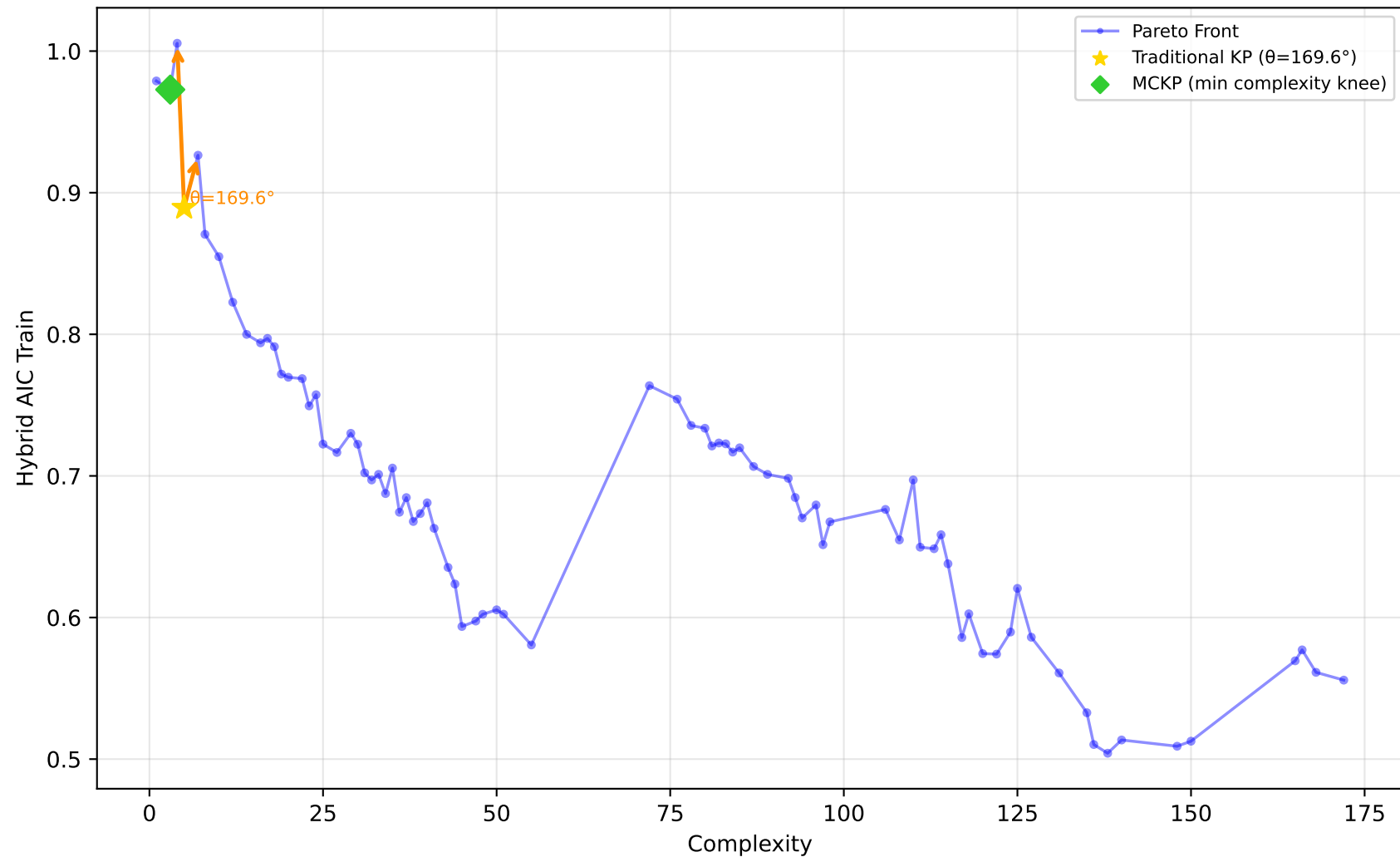
542_pollution - Run 24 - SVP - Hybrid AIC Train \lambda_1=0.00, \lambda_2=0.00, \lambda_3=0.20 | Difficulty: 0.39 | Method: mckp
