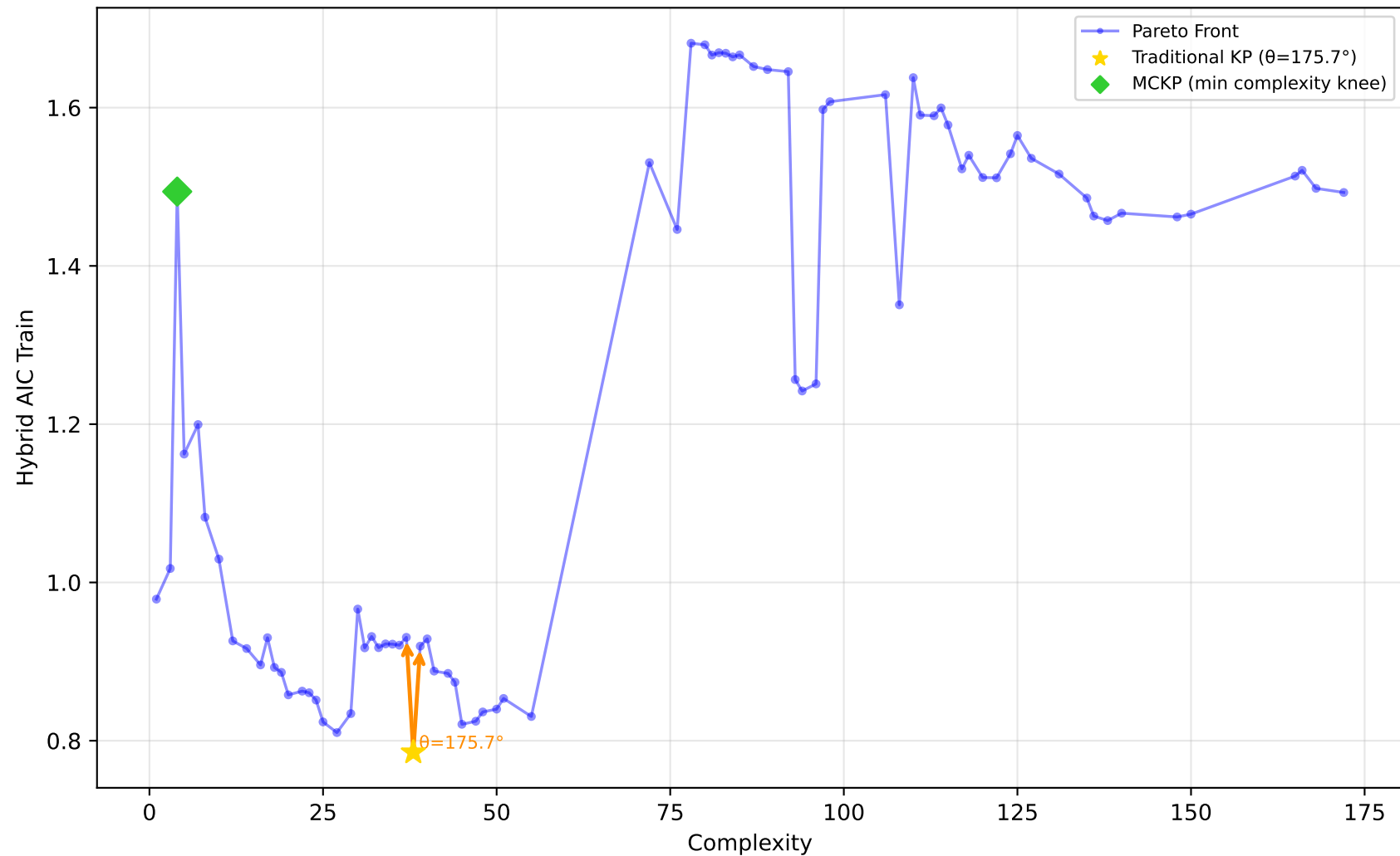
542_pollution - Run 24 - SVP - Hybrid AIC Train \lambda_1=0.70 , \lambda_2=1.00 , \lambda_3=0.10 | Difficulty: 0.39 | Method: mckp
