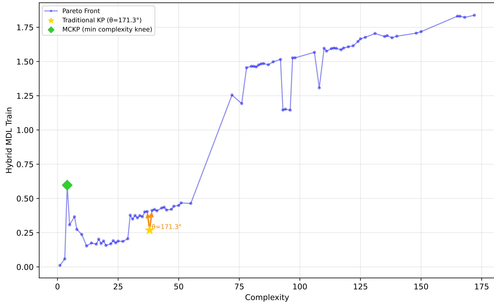
542_pollution - Run 24 - SVP - Hybrid MDL Train \lambda_1=0.70, \lambda_2=1.00, \lambda_3=0.10 | Difficulty: 0.39 | Method: mckp
