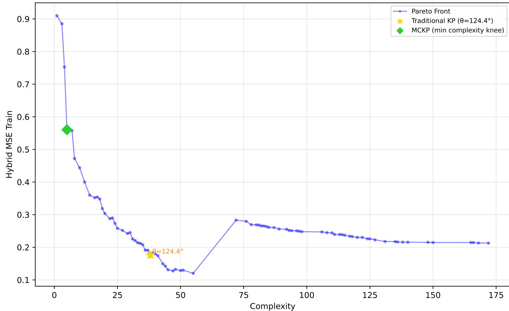
542_pollution - Run 24 - SVP - Hybrid MSE Train \lambda_1=0.00, \lambda_2=0.00, \lambda_3=0.20 | Difficulty: 0.39 | Method: mckp
