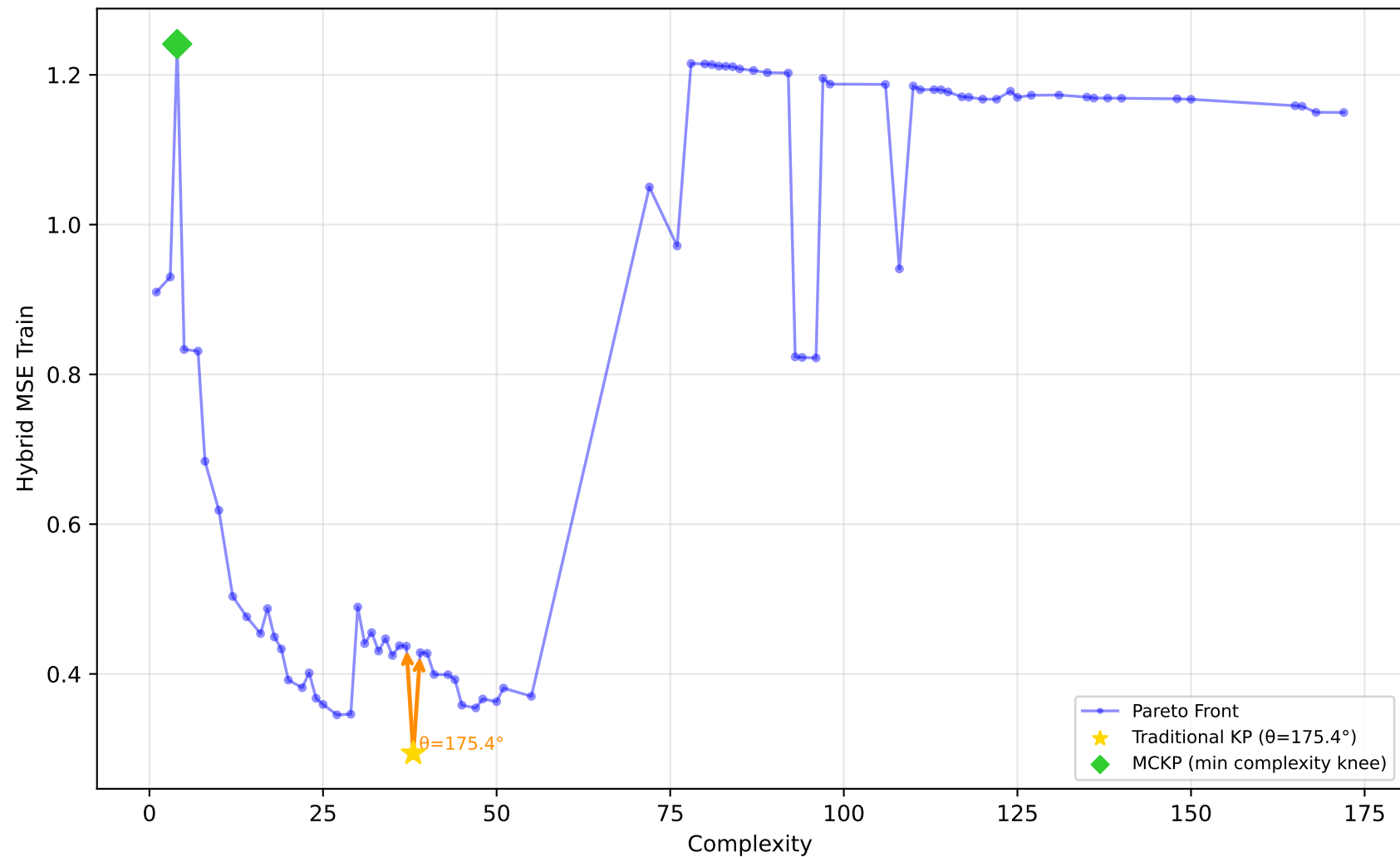
542_pollution - Run 24 - SVP - Hybrid MSE Train \lambda_1=0.70, \lambda_2=1.00, \lambda_3=0.10 | Difficulty: 0.39 | Method: mckp
