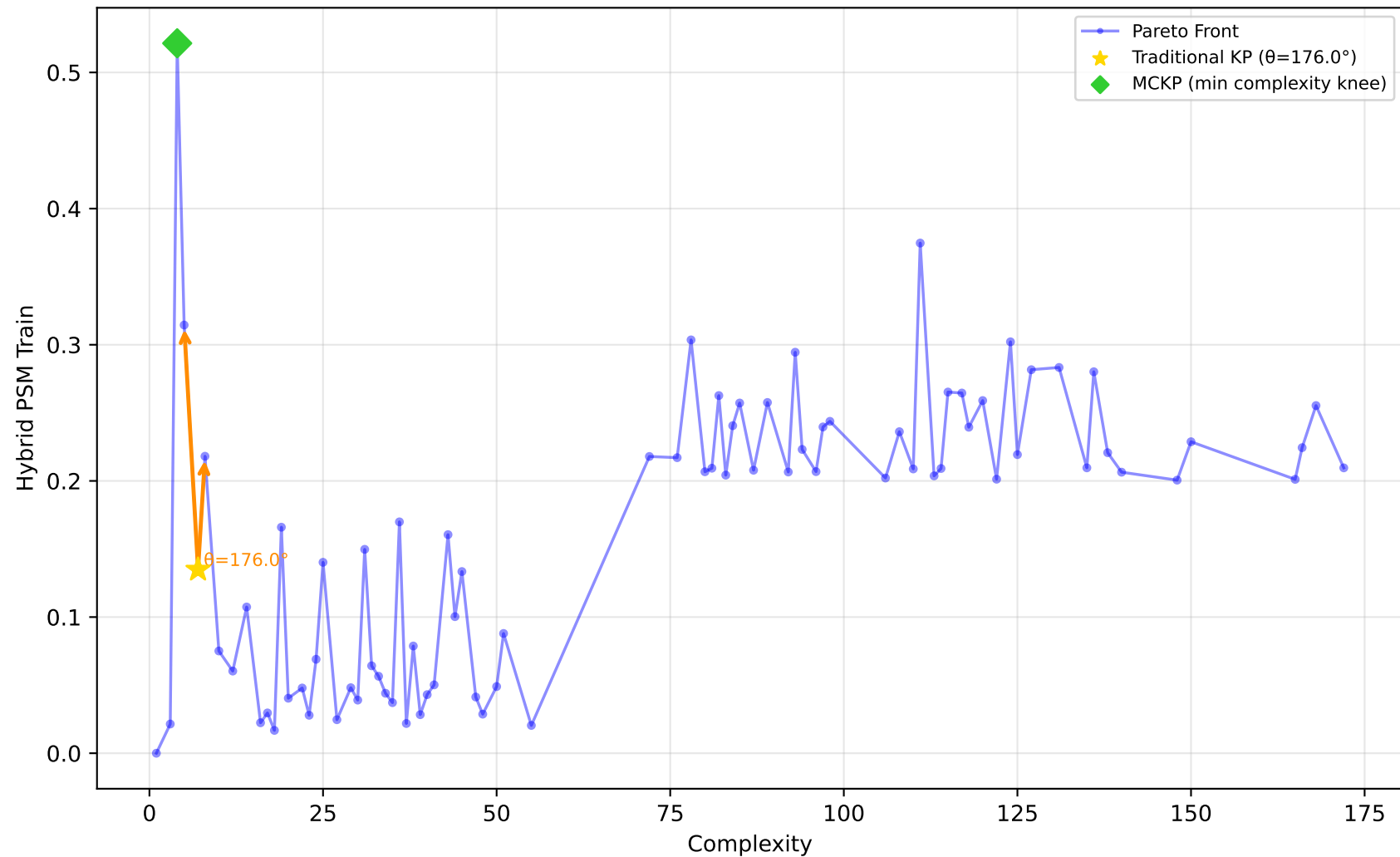
542_pollution - Run 24 - SVP - Hybrid PSM Train \lambda_1=0.00, \lambda_2=0.00, \lambda_3=0.20 | Difficulty: 0.39 | Method: mckp
