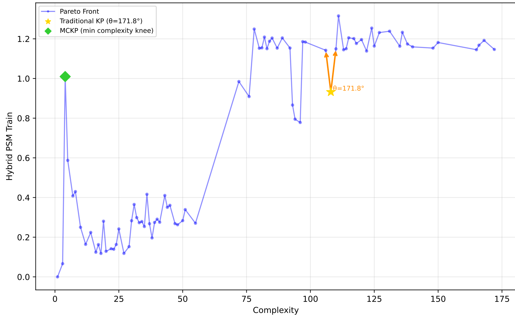
542_pollution - Run 24 - SVP - Hybrid PSM Train \lambda_1=0.70, \lambda_2=1.00, \lambda_3=0.10 | Difficulty: 0.39 | Method: mckp
