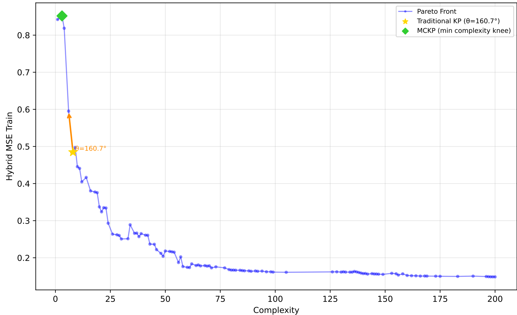
542_pollution - Run 25 - MVP - Hybrid MSE Train \lambda_1=0.40, \lambda_2=0.10, \lambda_3=0.00 | Difficulty: 0.16 | Method: mckp
