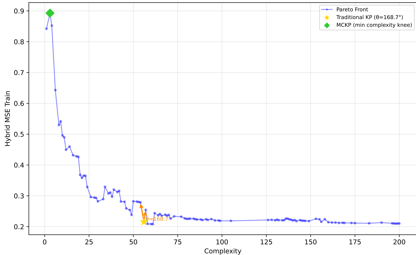
542_pollution - Run 25 - MVP - Hybrid MSE Train \lambda_1=1.00, \lambda_2=0.10, \lambda_3=0.00 | Difficulty: 0.16 | Method: mckp
