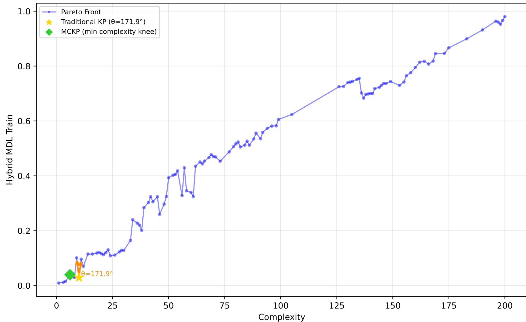
542_pollution - Run 25 - SVP - Hybrid MDL Train \lambda_1=0.00, \lambda_2=0.00, \lambda_3=0.20 | Difficulty: 0.16 | Method: mckp
