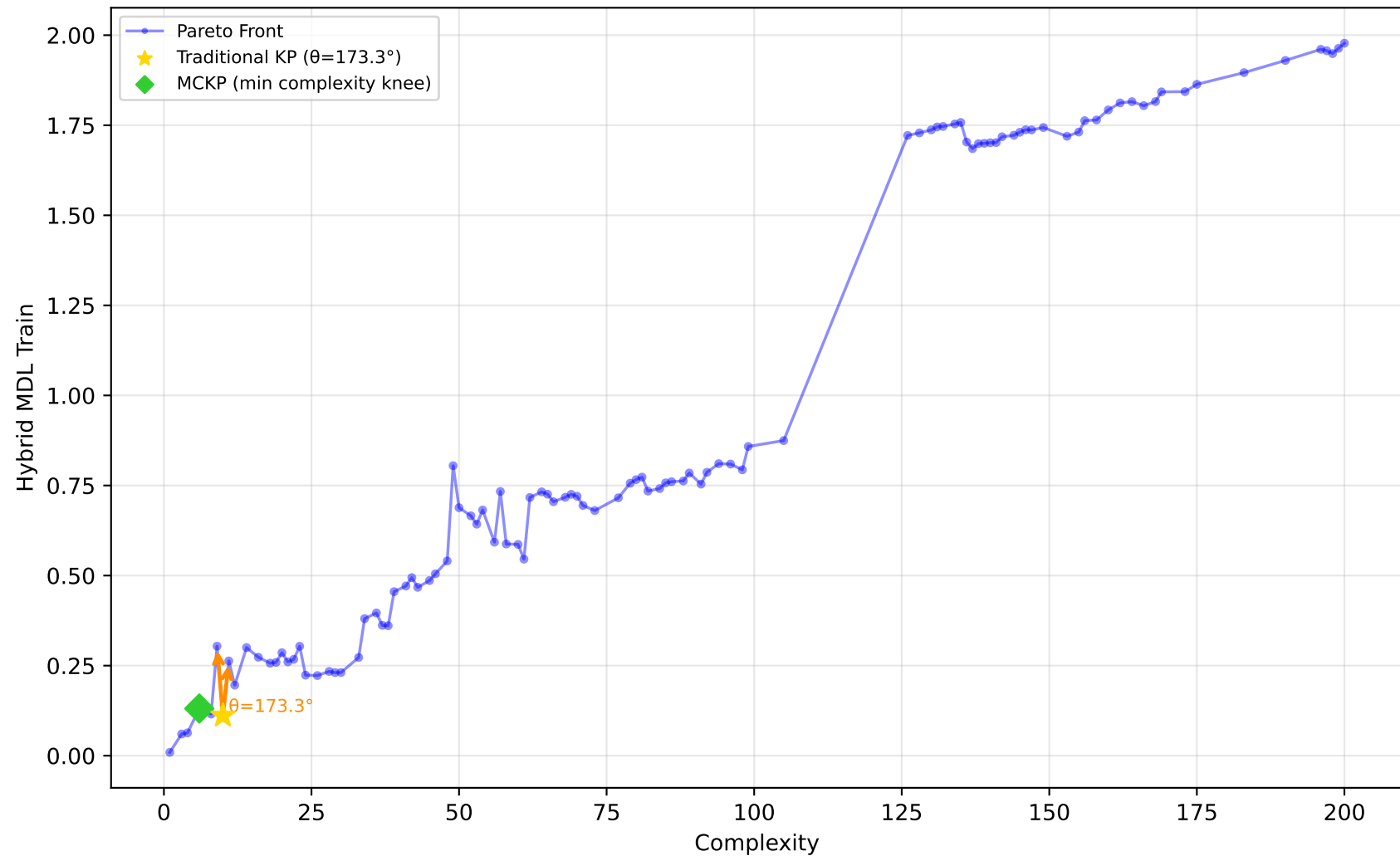
542_pollution - Run 25 - SVP - Hybrid MDL Train \lambda_1=0.70, \lambda_2=1.00, \lambda_3=0.10 | Difficulty: 0.16 | Method: mckp
