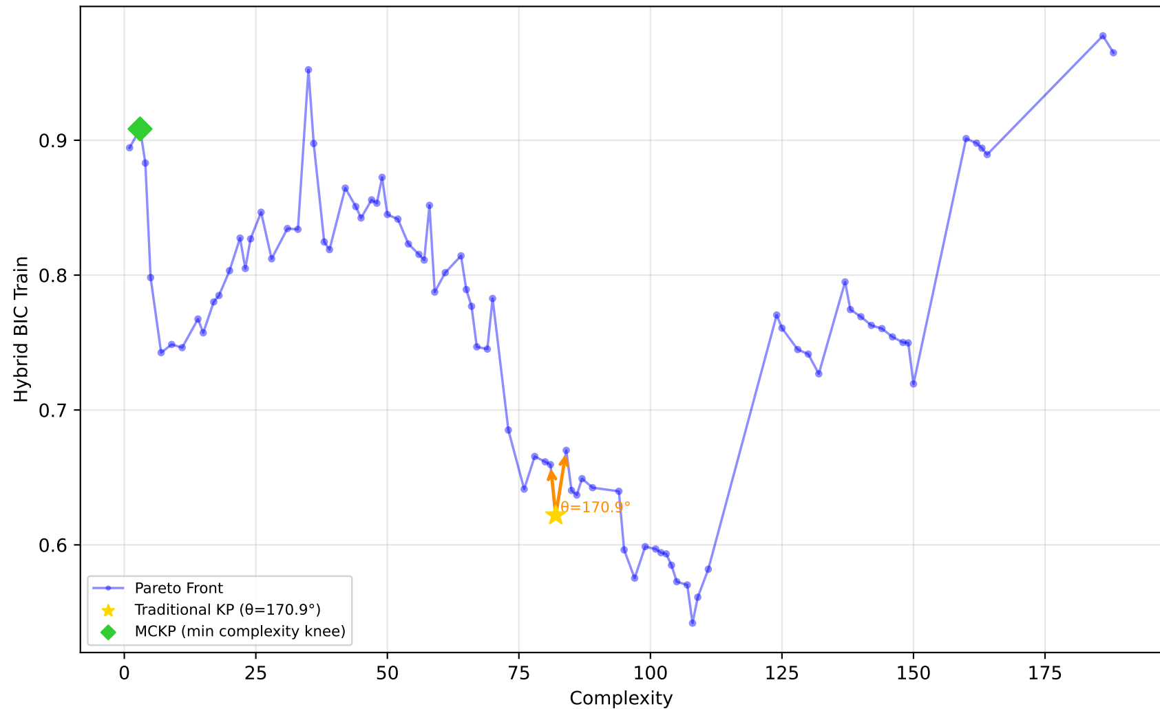
542_pollution - Run 26 - MVP - Hybrid BIC Train \lambda_1=0.40, \lambda_2=0.10, \lambda_3=0.00 | Difficulty: 0.29 | Method: mckp
