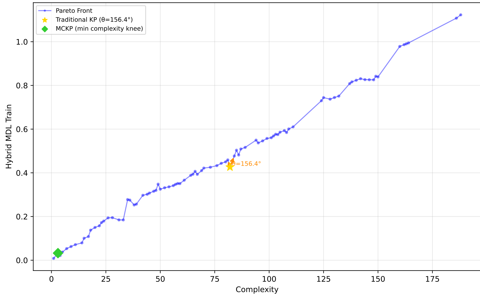
542_pollution - Run 26 - MVP - Hybrid MDL Train \lambda_1=0.40, \lambda_2=0.10, \lambda_3=0.00 | Difficulty: 0.29 | Method: mckp
