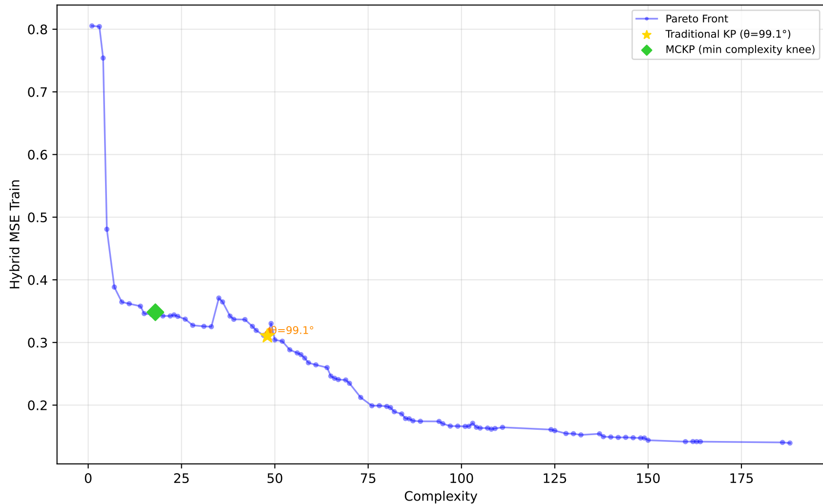
542_pollution - Run 26 - MVP - Hybrid MSE Train \lambda_1=0.40, \lambda_2=0.10, \lambda_3=0.00 | Difficulty: 0.29 | Method: mckp
