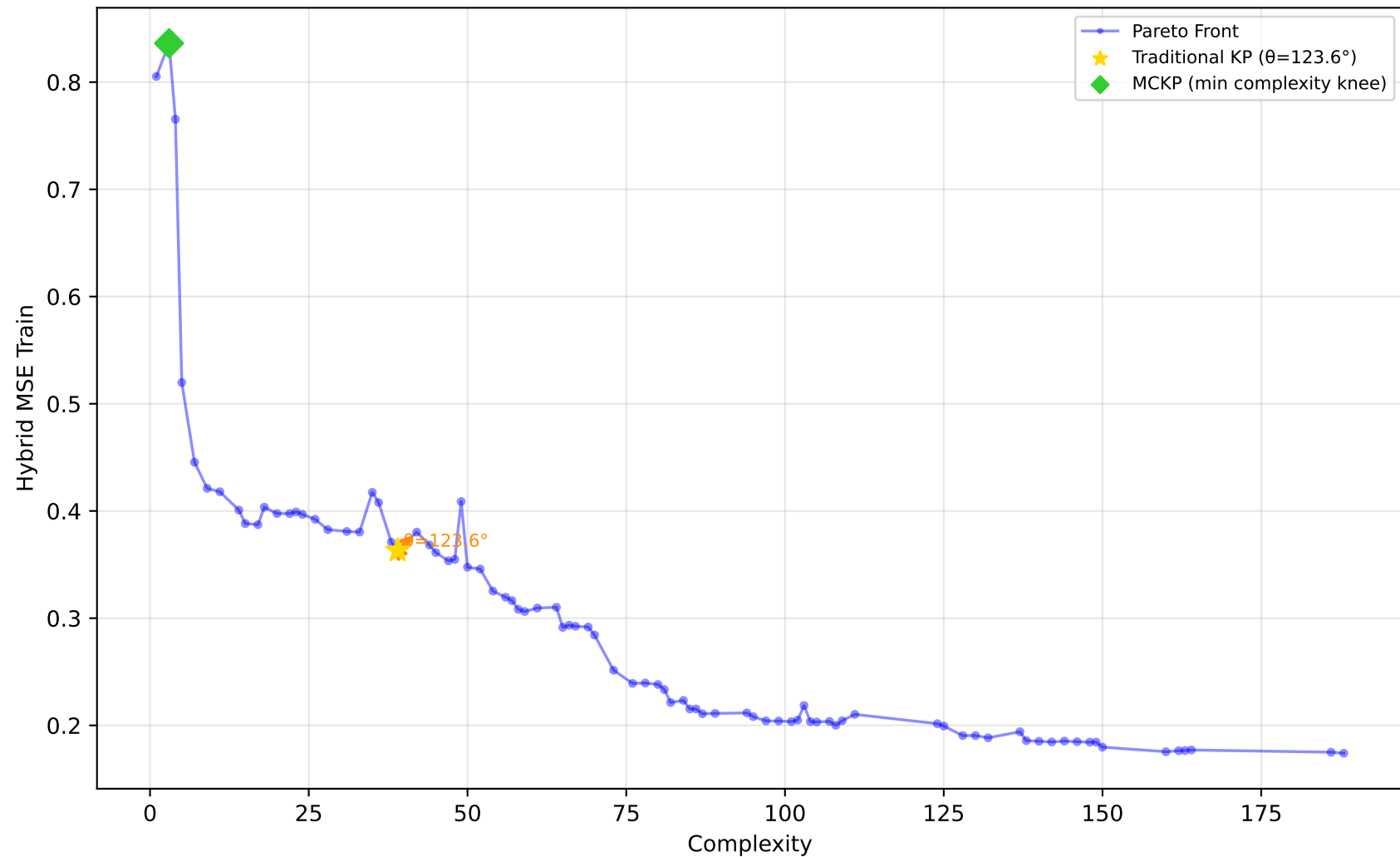
542_pollution - Run 26 - MVP - Hybrid MSE Train \lambda_1=1.00, \bar{\lambda}_2=0.10, \lambda_3=0.00 | Difficulty: 0.29 | Method: mckp
