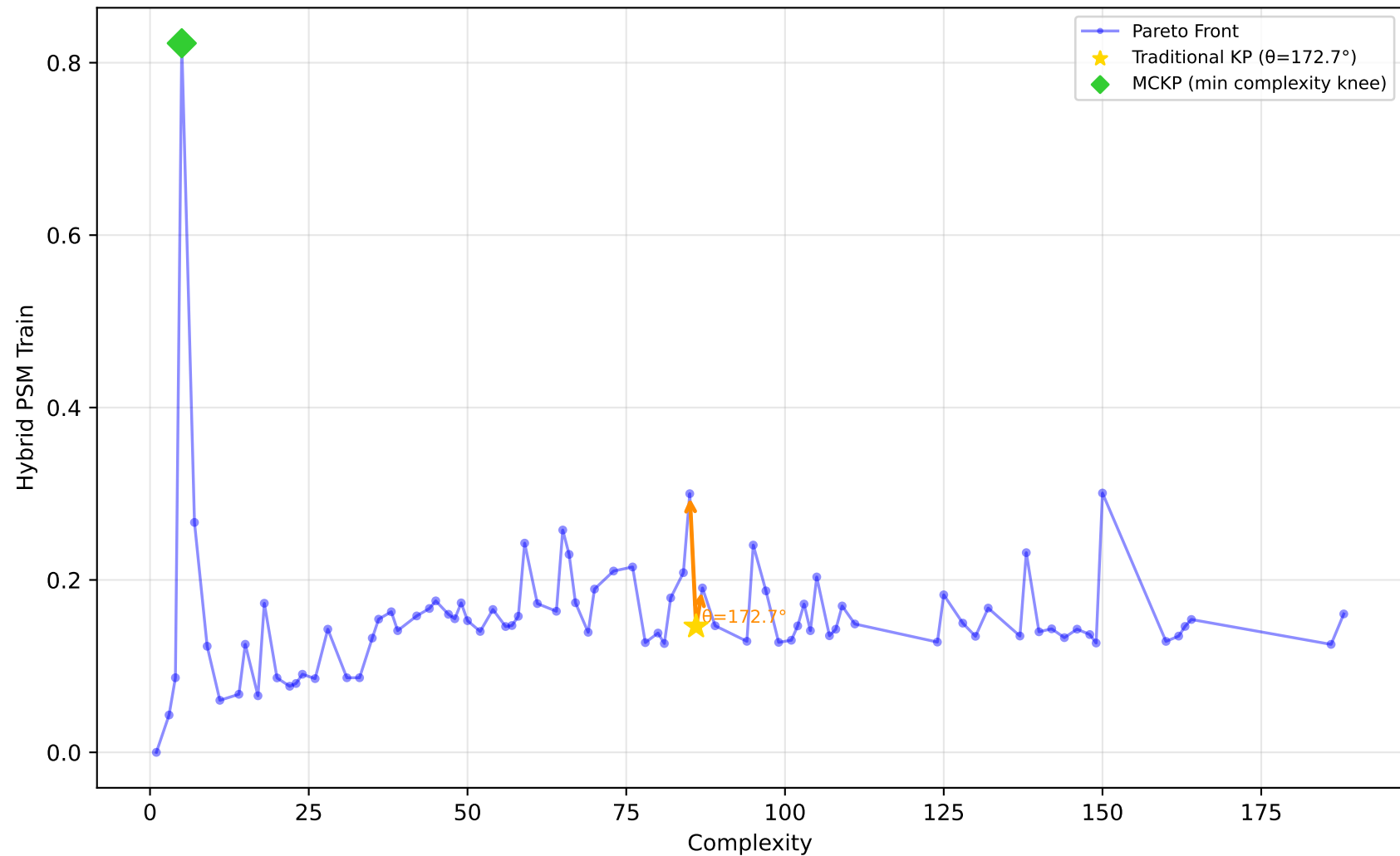
542_pollution - Run 26 - MVP - Hybrid PSM Train \lambda_1=0.40, \lambda_2=0.10, \lambda_3=0.00 | Difficulty: 0.29 | Method: mckp
