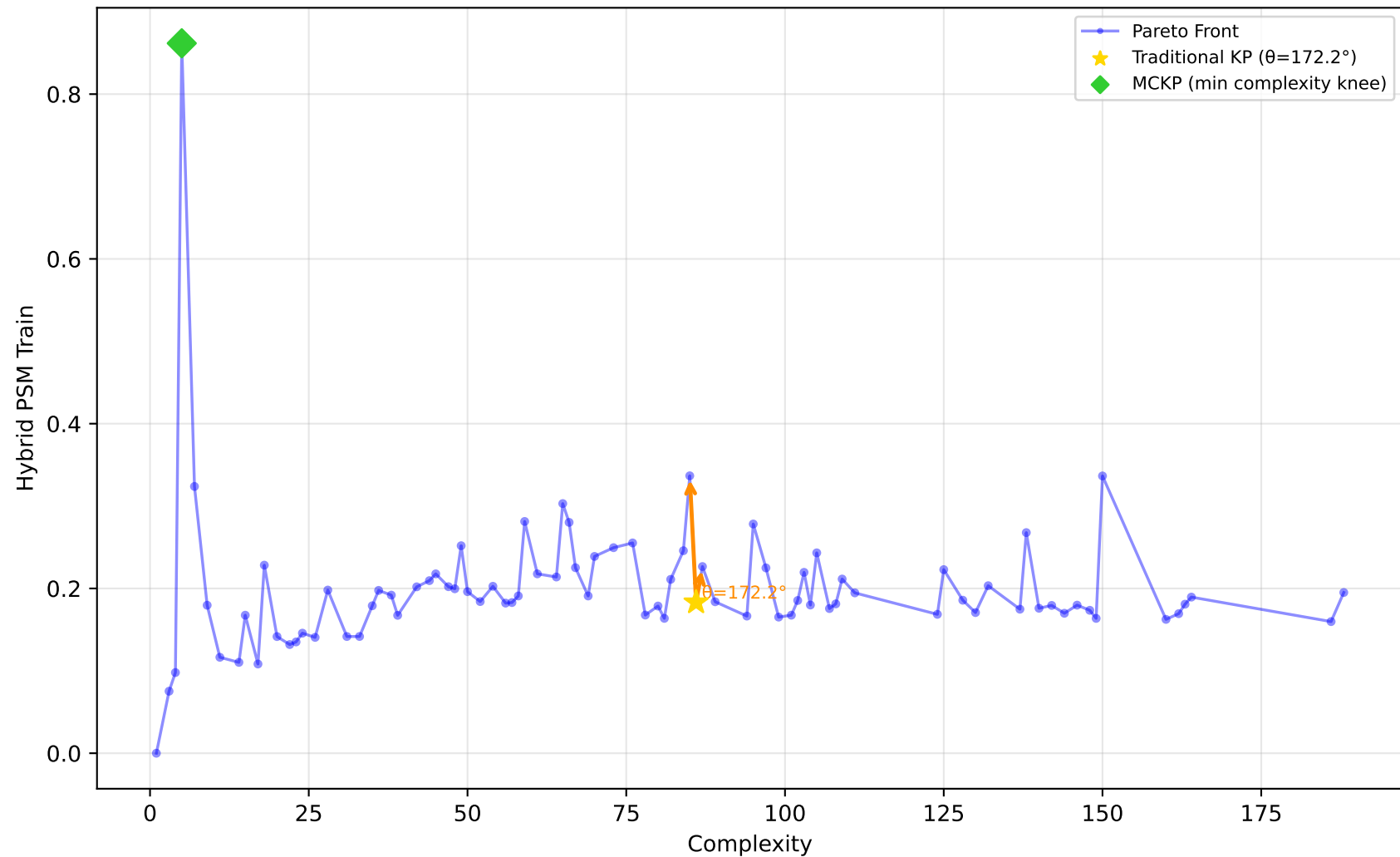
542_pollution - Run 26 - MVP - Hybrid PSM Train \lambda_1=1.00, \lambda_2=0.10, \lambda_3=0.00 | Difficulty: 0.29 | Method: mckp
