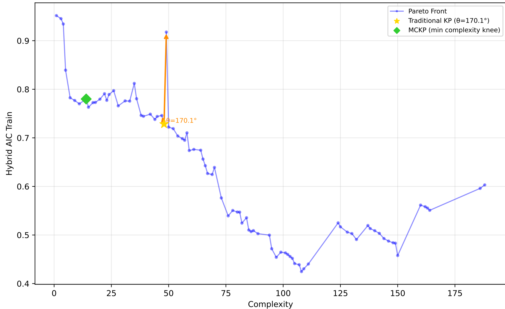
542_pollution - Run 26 - SVP - Hybrid AIC Train \lambda_1=0.00, \lambda_2=0.00, \lambda_3=0.20 | Difficulty: 0.29 | Method: mckp
