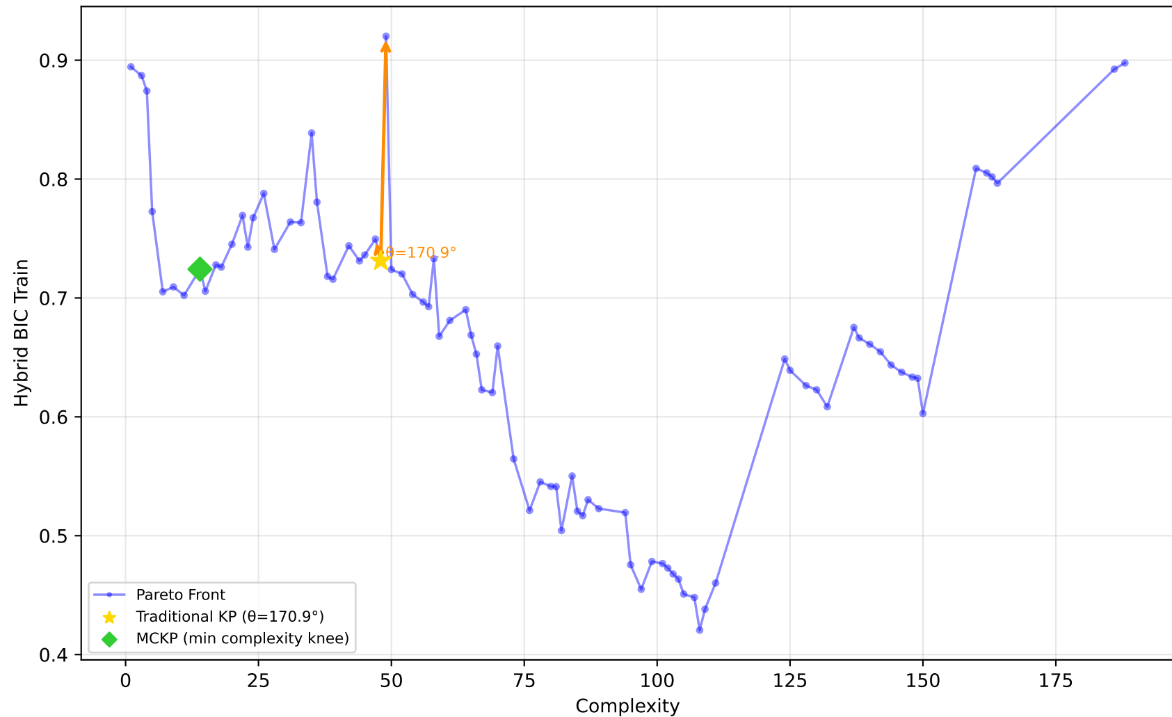
542_pollution - Run 26 - SVP - Hybrid BIC Train \lambda_1=0.00, \lambda_2=0.00, \lambda_3=0.20 | Difficulty: 0.29 | Method: mckp
