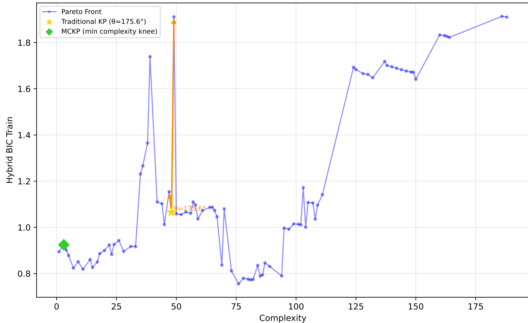
542_pollution - Run 26 - SVP - Hybrid BIC Train \lambda_1=0.70, \lambda_2=1.00, \lambda_3=0.10 | Difficulty: 0.29 | Method: mckp
