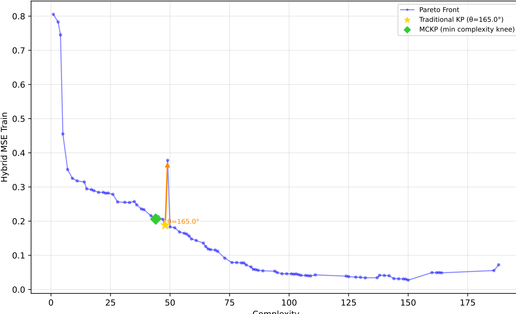
542_pollution - Run 26 - SVP - Hybrid MSE Train \lambda_1=0.00 , \lambda_2=0.00 , \lambda_3=0.20 | Difficulty: 0.29 | Method: mckp
