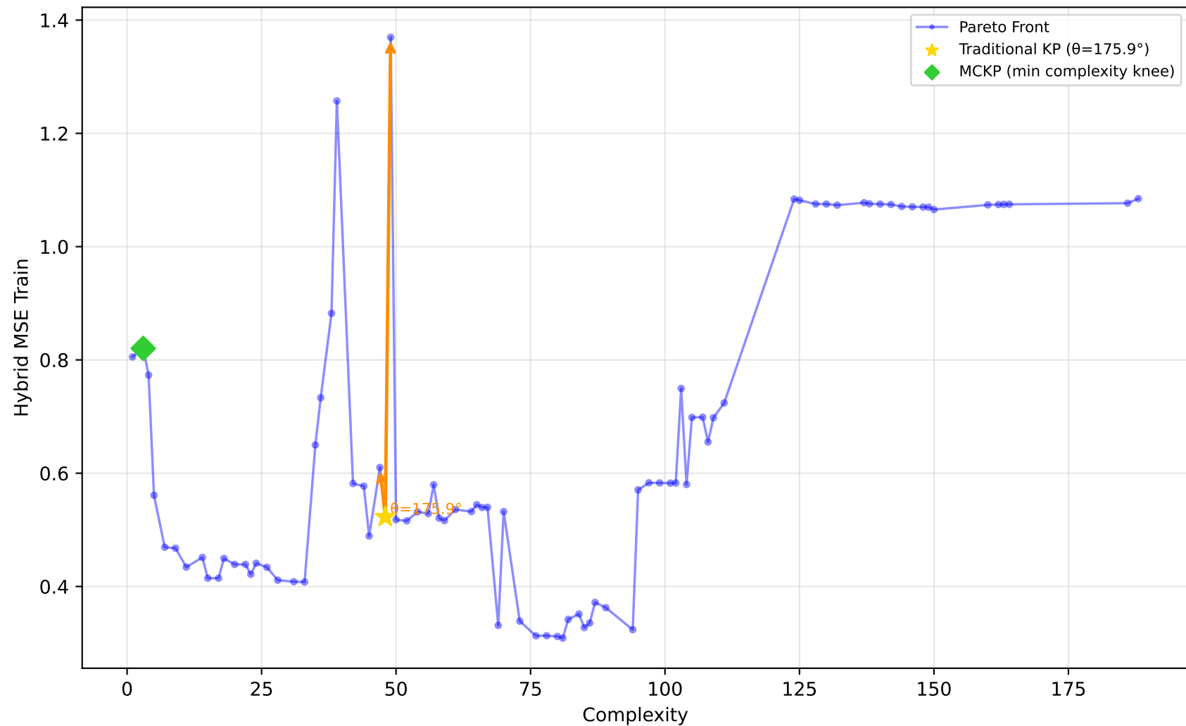
542_pollution - Run 26 - SVP - Hybrid MSE Train \lambda_1=0.70, \lambda_2=1.00, \lambda_3=0.10 | Difficulty: 0.29 | Method: mckp
