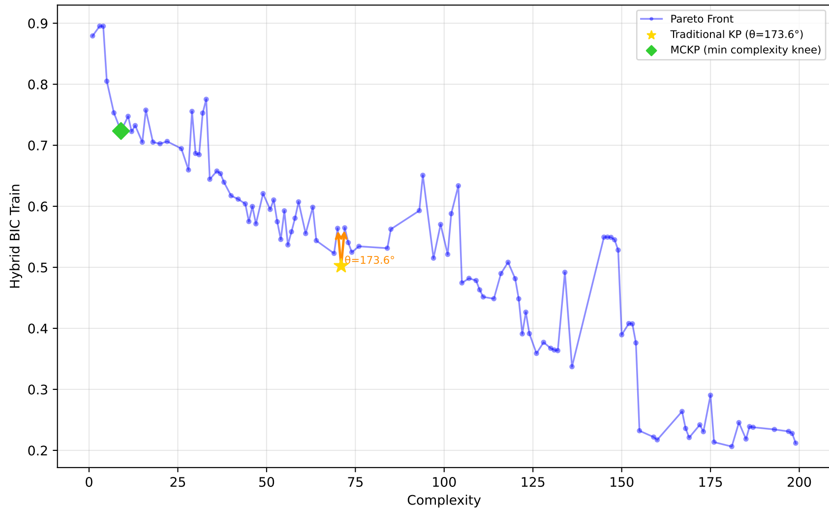
542_pollution - Run 27 - MVP - Hybrid BIC Train \lambda_1=0.40, \lambda_2=0.10, \lambda_3=0.00 | Difficulty: 0.33 | Method: mckp
