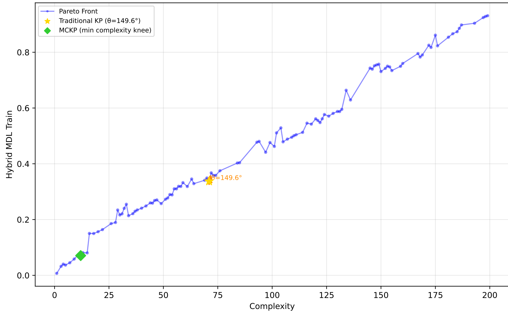
542_pollution - Run 27 - MVP - Hybrid MDL Train \lambda_1=0.40, \bar{\lambda}_2=0.10, \lambda_3=0.00 | Difficulty: 0.33 | Method: mckp
