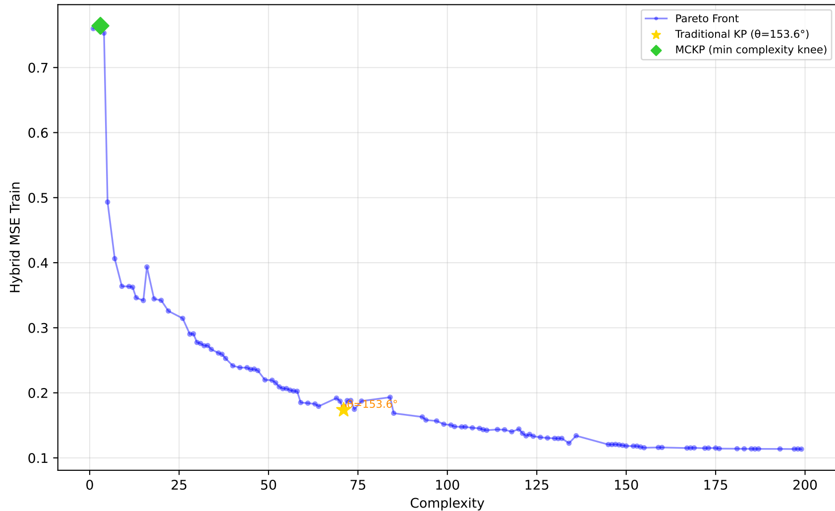
542_pollution - Run 27 - MVP - Hybrid MSE Train \lambda_1=0.40, \lambda_2=0.10, \lambda_3=0.00 | Difficulty: 0.33 | Method: mckp
