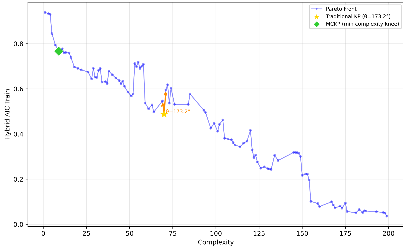
542_pollution - Run 27 - SVP - Hybrid AIC Train \lambda_1=0.00, \lambda_2=0.00, \lambda_3=0.20 | Difficulty: 0.33 | Method: mckp
