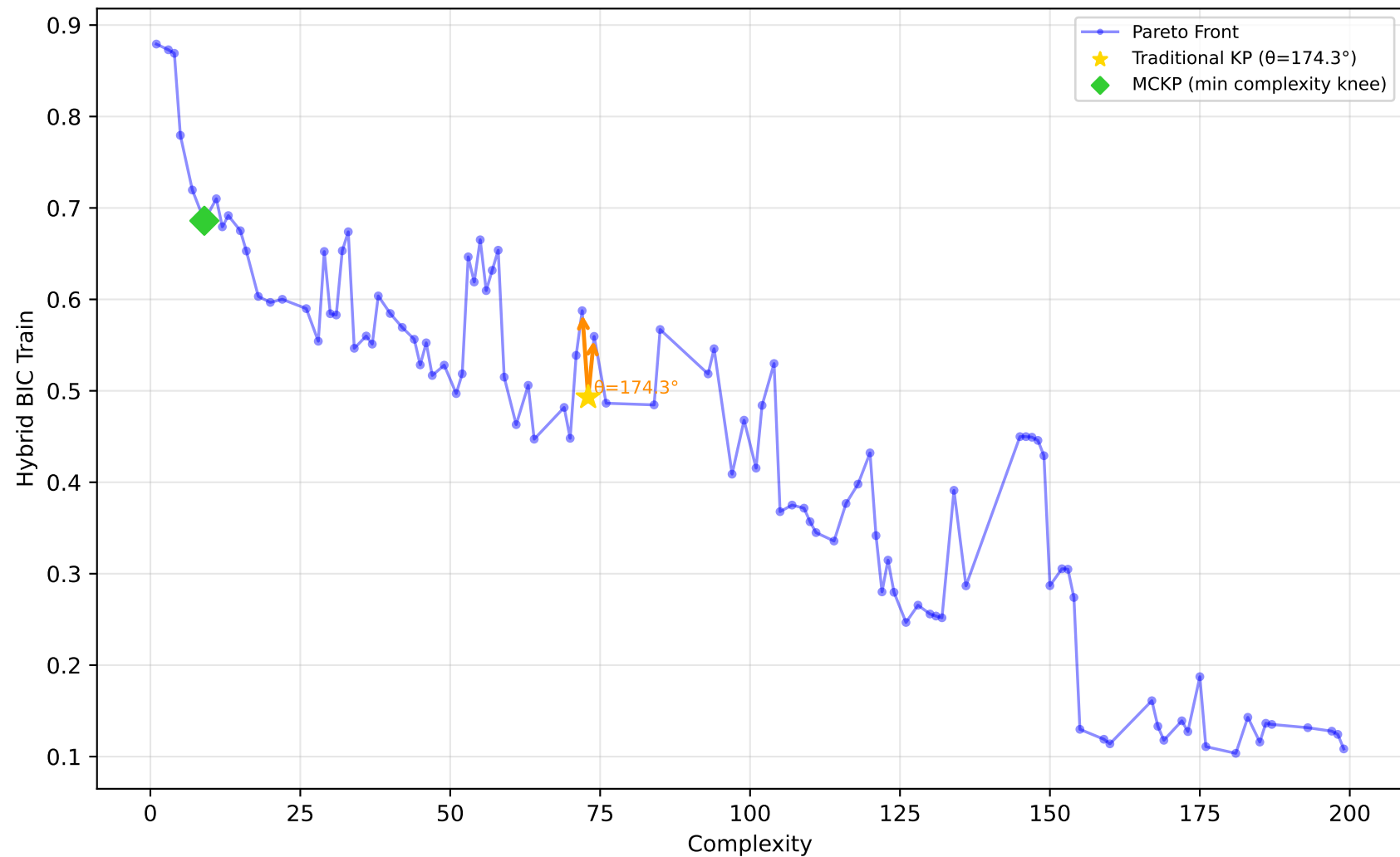
542_pollution - Run 27 - SVP - Hybrid BIC Train \lambda_1=0.00, \lambda_2=0.00, \lambda_3=0.20 | Difficulty: 0.33 | Method: mckp
