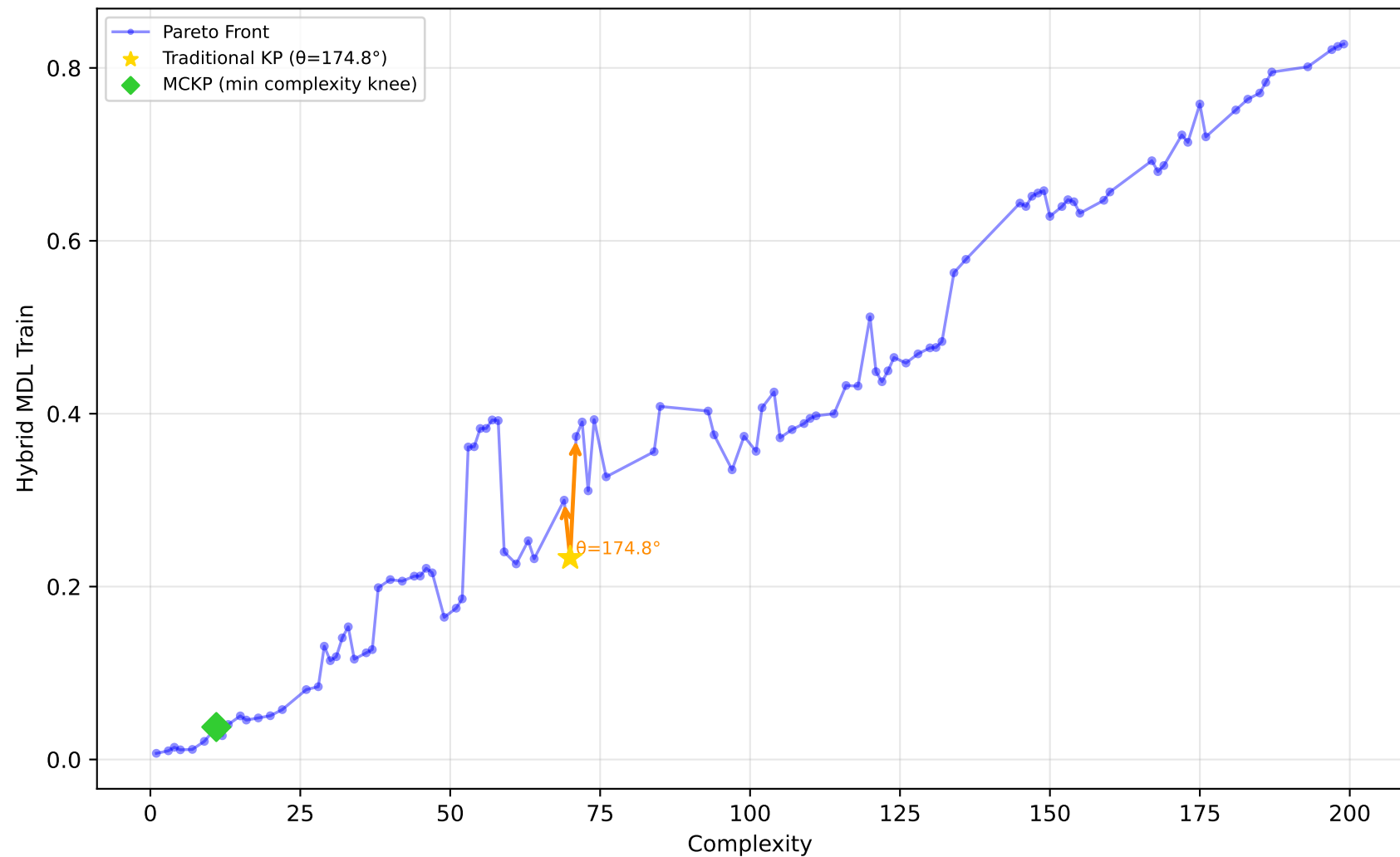
542_pollution - Run 27 - SVP - Hybrid MDL Train \lambda_1=0.00, \lambda_2=0.00, \lambda_3=0.20 | Difficulty: 0.33 | Method: mckp
