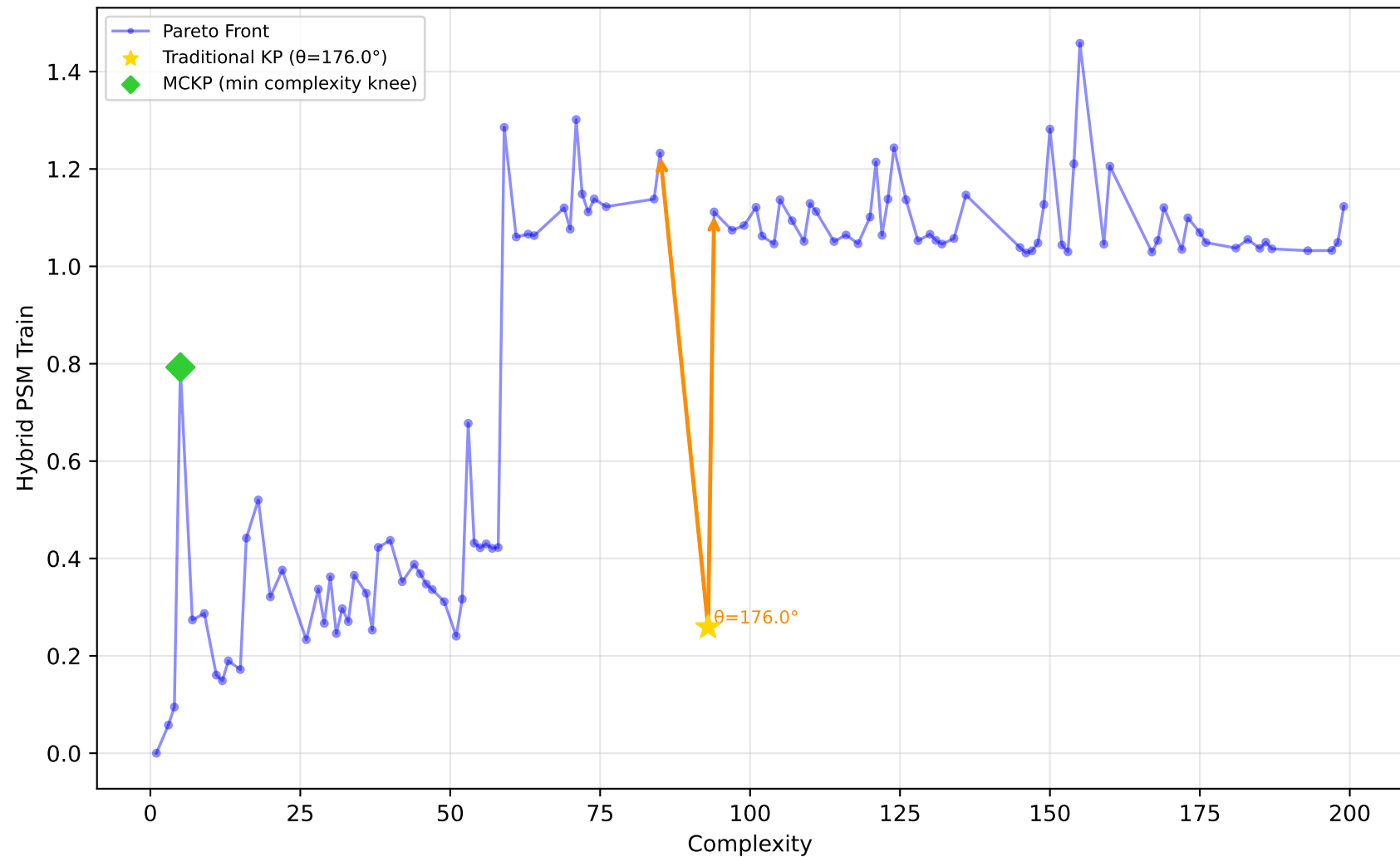
542_pollution - Run 27 - SVP - Hybrid PSM Train \lambda_1=0.70, \lambda_2=1.00, \lambda_3=0.10 | Difficulty: 0.33 | Method: mckp
