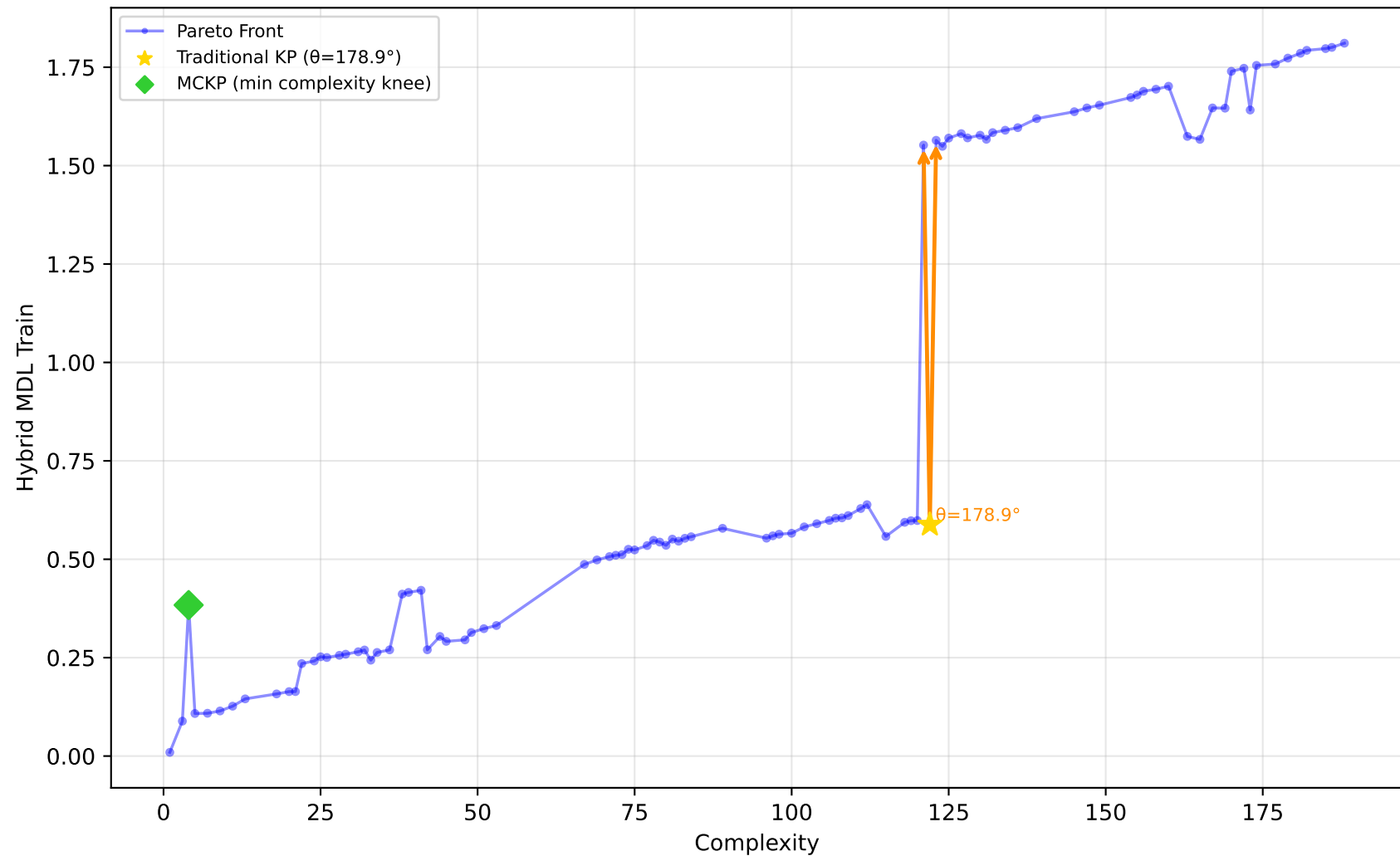
542_pollution - Run 28 - MVP - Hybrid MDL Train \lambda_1=1.00, \lambda_2=0.10, \lambda_3=0.00 | Difficulty: 0.41 | Method: mckp
