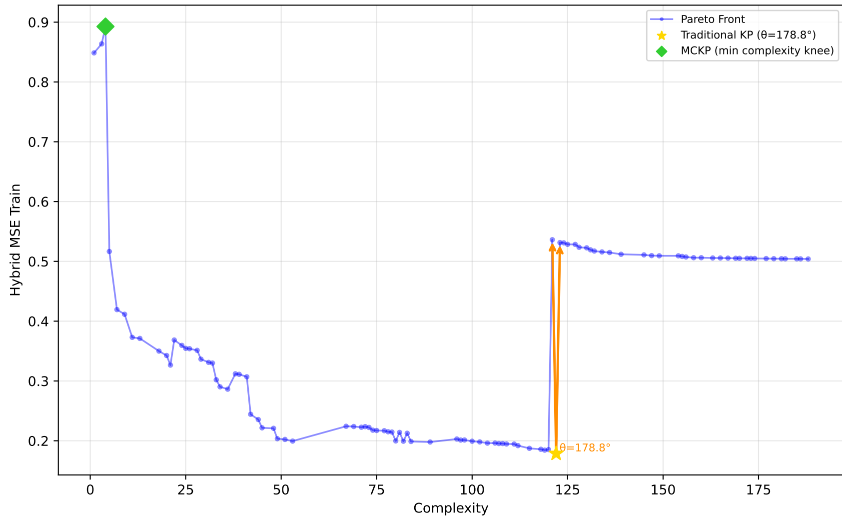
542_pollution - Run 28 - MVP - Hybrid MSE Train \lambda_1=0.40, \lambda_2=0.10, \lambda_3=0.00 | Difficulty: 0.41 | Method: mckp
