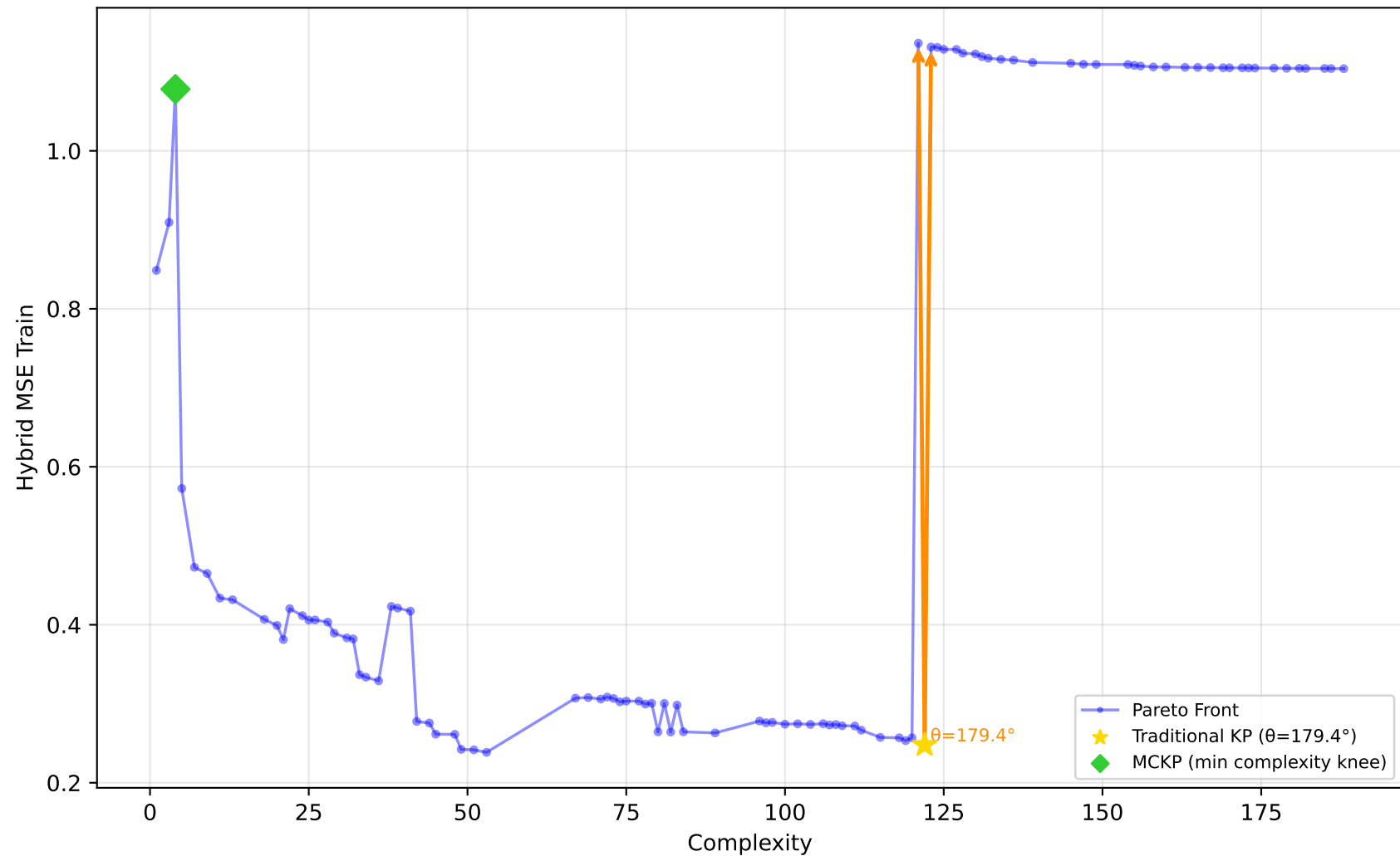
542_pollution - Run 28 - MVP - Hybrid MSE Train \lambda_1=1.00, \lambda_2=0.10, \lambda_3=0.00 | Difficulty: 0.41 | Method: mckp
