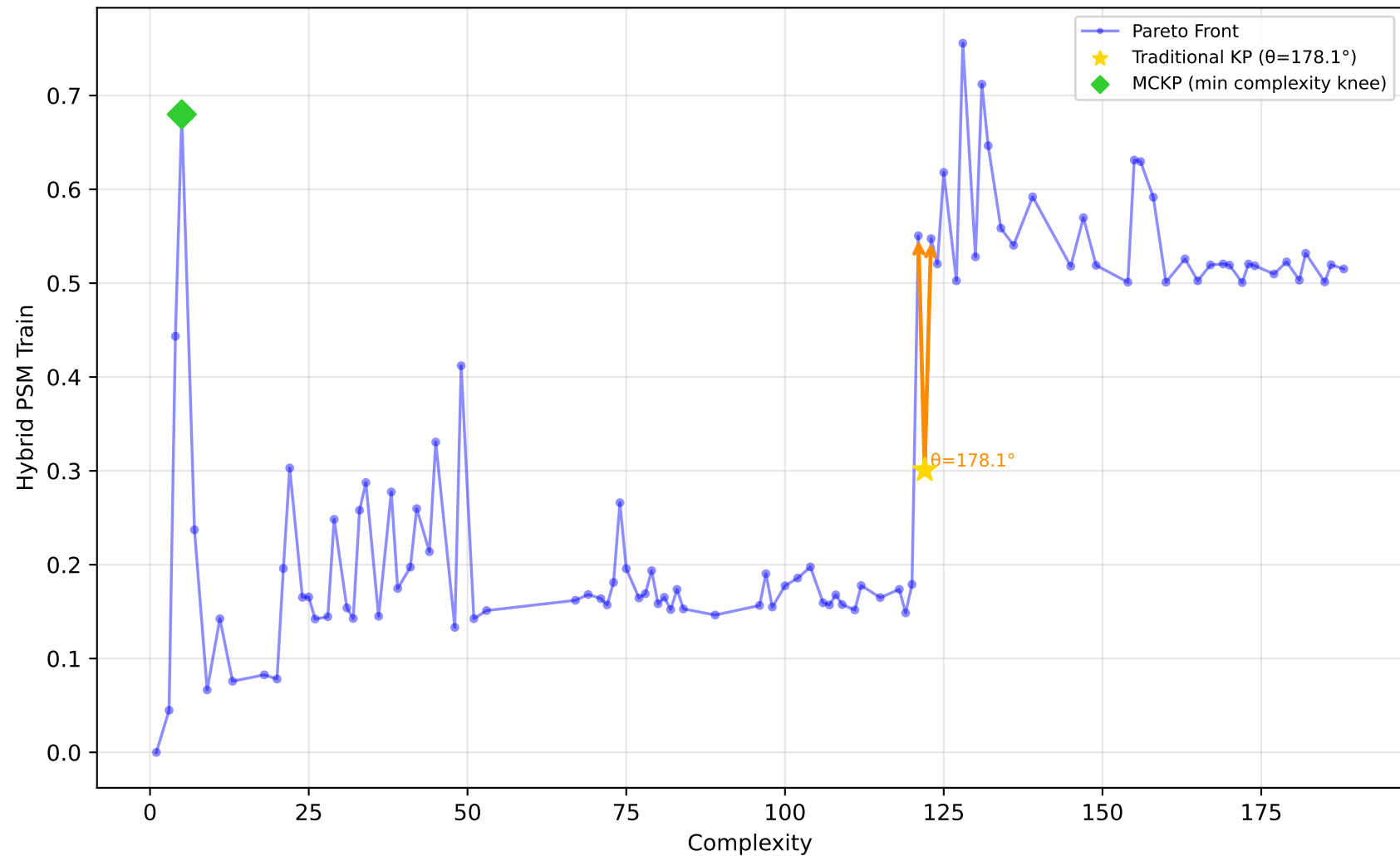
542_pollution - Run 28 - MVP - Hybrid PSM Train \lambda_1=0.40, \lambda_2=0.10, \lambda_3=0.00 | Difficulty: 0.41 | Method: mckp
