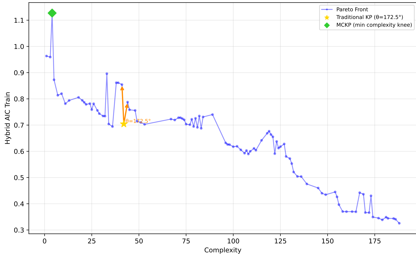
542_pollution - Run 28 - SVP - Hybrid AIC Train \lambda_1=0.00, \lambda_2=0.00, \lambda_3=0.20 | Difficulty: 0.41 | Method: mckp
