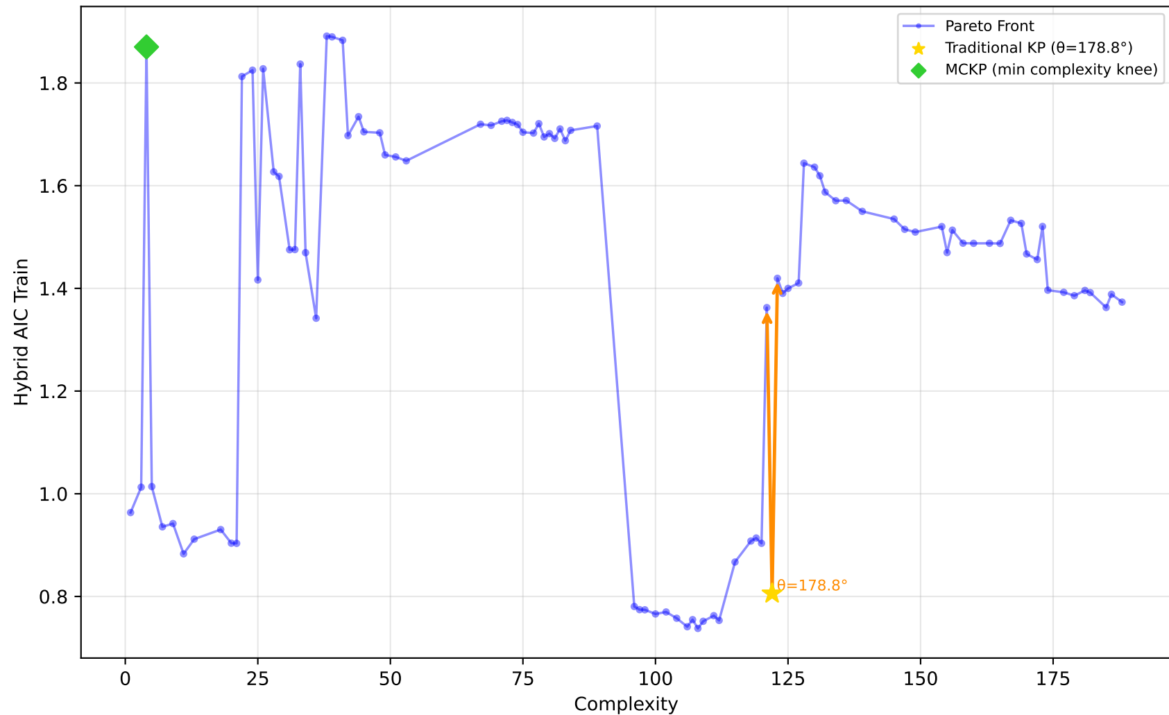
542_pollution - Run 28 - SVP - Hybrid AIC Train \lambda_1=0.70 , \lambda_2=1.00 , \lambda_3=0.10 | Difficulty: 0.41 | Method: mckp
