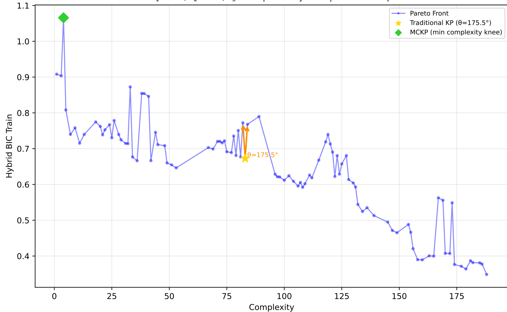
542_pollution - Run 28 - SVP - Hybrid BIC Train \lambda_1=0.00, \lambda_2=0.00, \lambda_3=0.20 | Difficulty: 0.41 | Method: mckp
