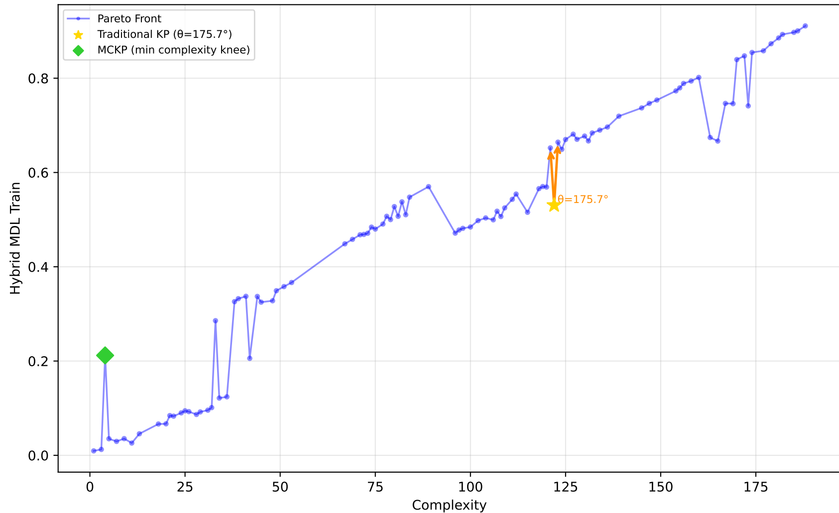
542_pollution - Run 28 - SVP - Hybrid MDL Train \lambda_1=0.00, \lambda_2=0.00, \lambda_3=0.20 | Difficulty: 0.41 | Method: mckp
