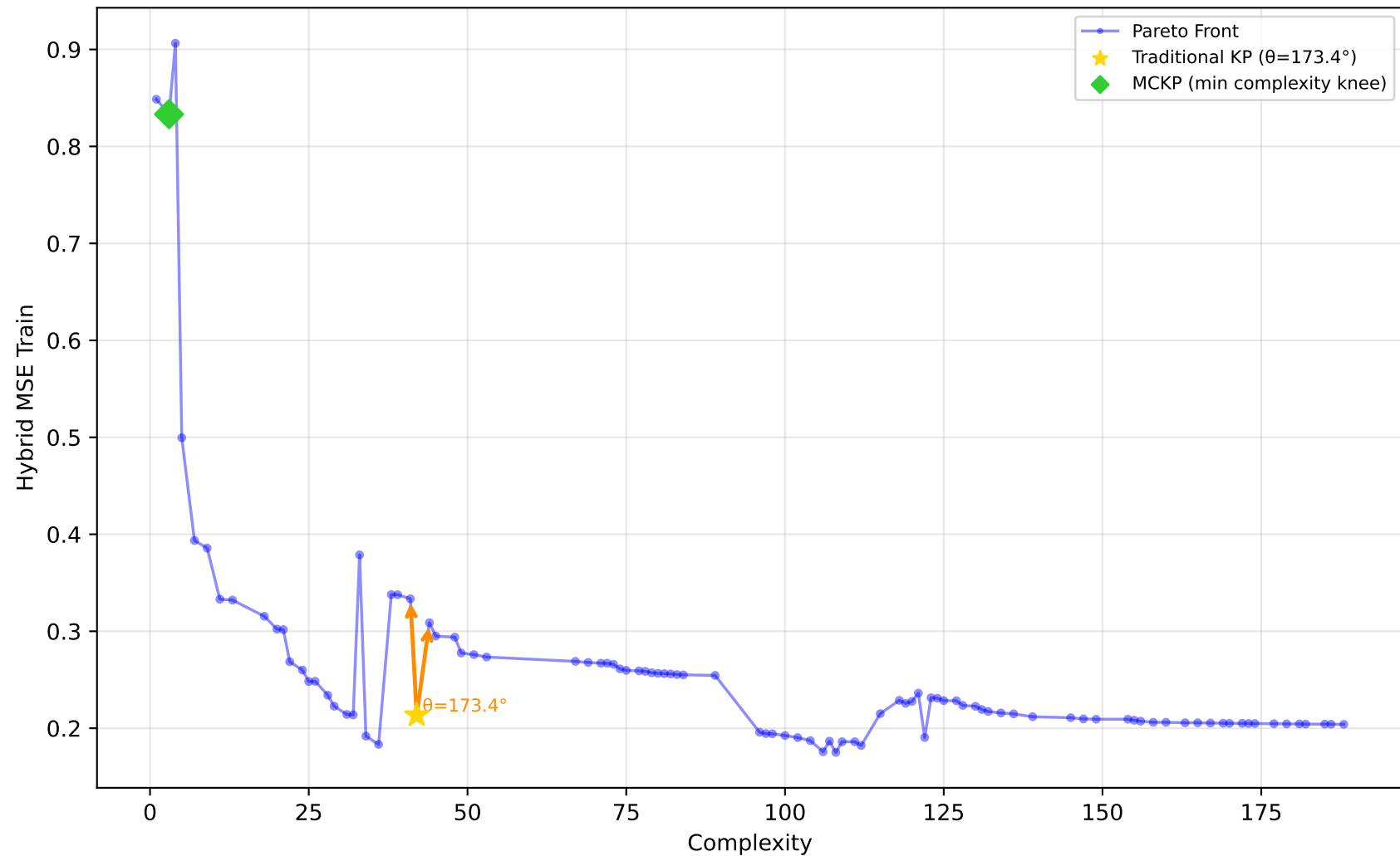
542_pollution - Run 28 - SVP - Hybrid MSE Train \lambda_1=0.00, \lambda_2=0.00, \lambda_3=0.20 | Difficulty: 0.41 | Method: mckp
