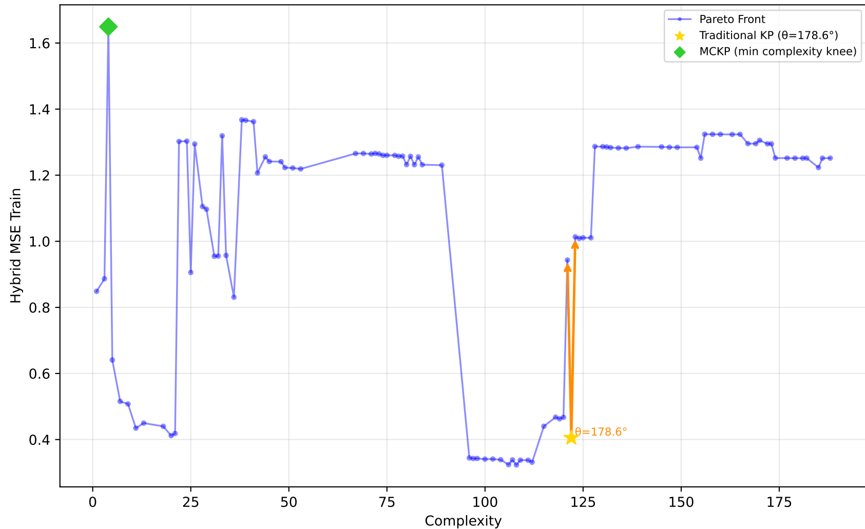
542_pollution - Run 28 - SVP - Hybrid MSE Train \lambda_1=0.70 , \lambda_2=1.00 , \lambda_3=0.10 | Difficulty: 0.41 | Method: mckp
