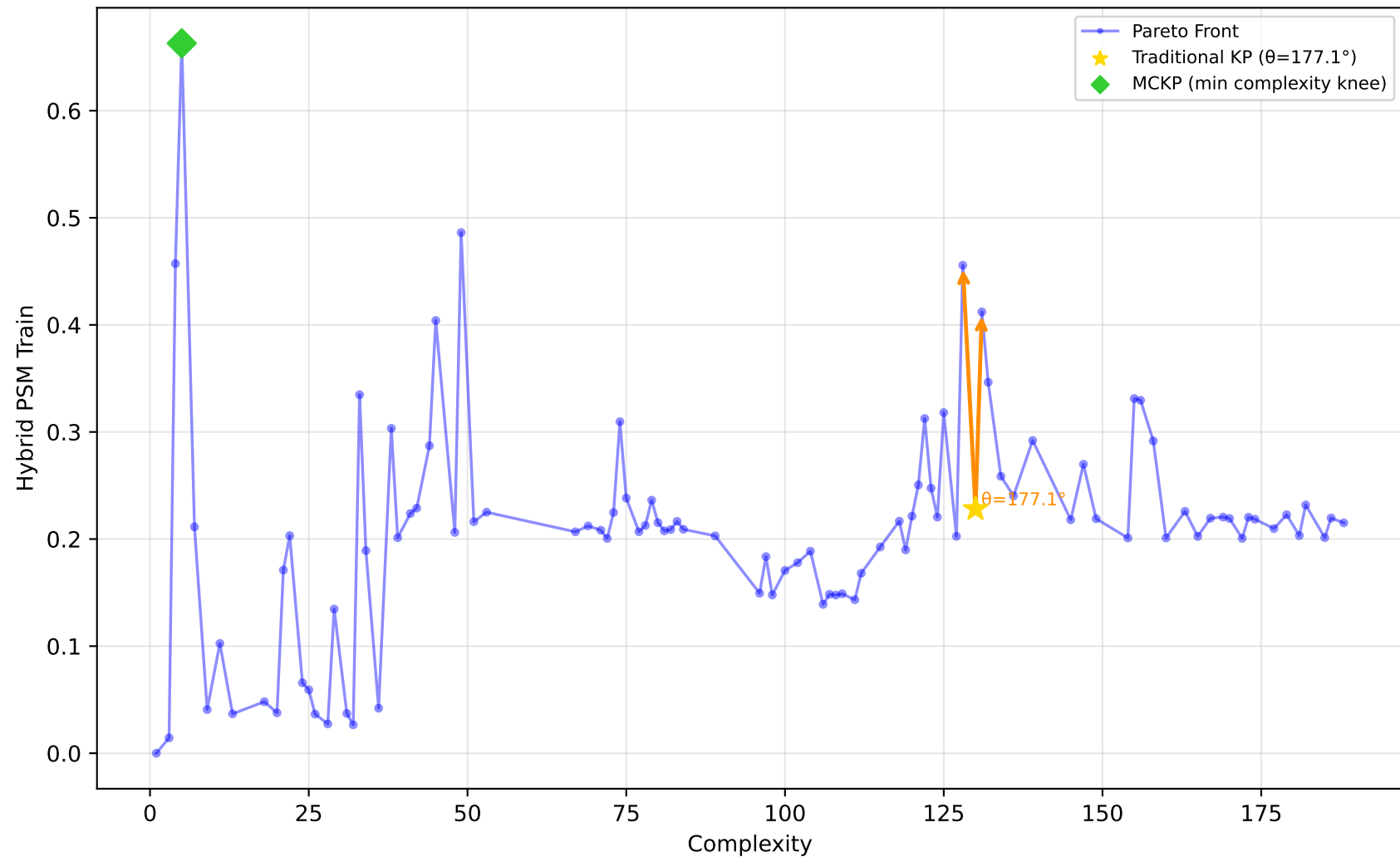
542_pollution - Run 28 - SVP - Hybrid PSM Train \lambda_1=0.00, \lambda_2=0.00, \lambda_3=0.20 | Difficulty: 0.41 | Method: mckp
