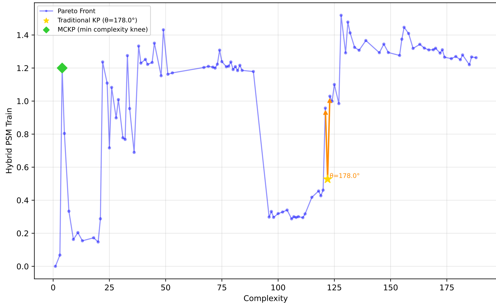
542_pollution - Run 28 - SVP - Hybrid PSM Train \lambda_1=0.70 , \lambda_2=1.00 , \lambda_3=0.10 | Difficulty: 0.41 | Method: mckp
