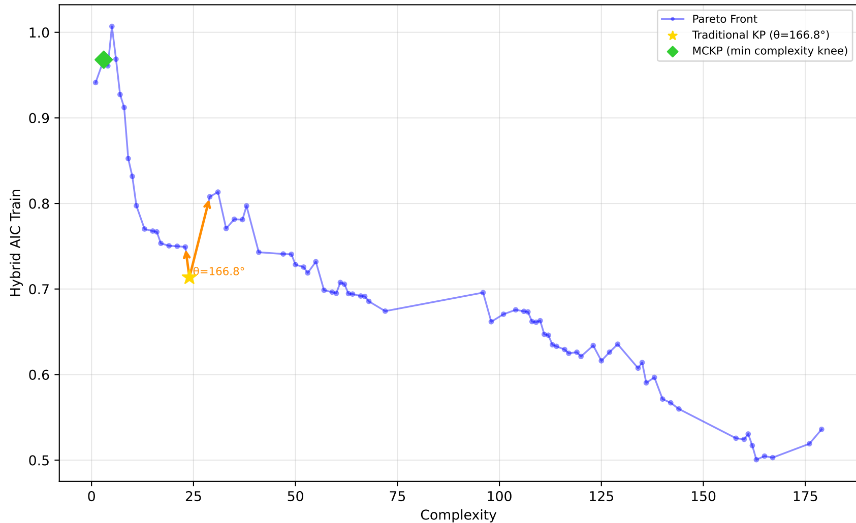
542_pollution - Run 29 - MVP - Hybrid AIC Train \lambda_1=0.40, \lambda_2=0.10, \lambda_3=0.00 | Difficulty: 1.00 | Method: hmr
