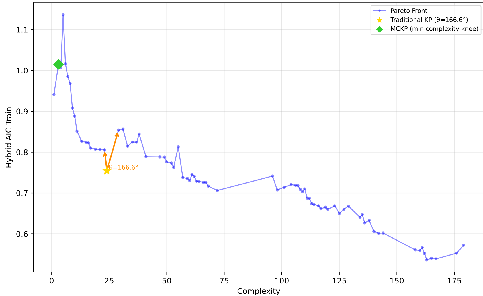
542_pollution - Run 29 - MVP - Hybrid AIC Train \lambda_1=1.00, \lambda_2=0.10, \lambda_3=0.00 | Difficulty: 1.00 | Method: hmr
