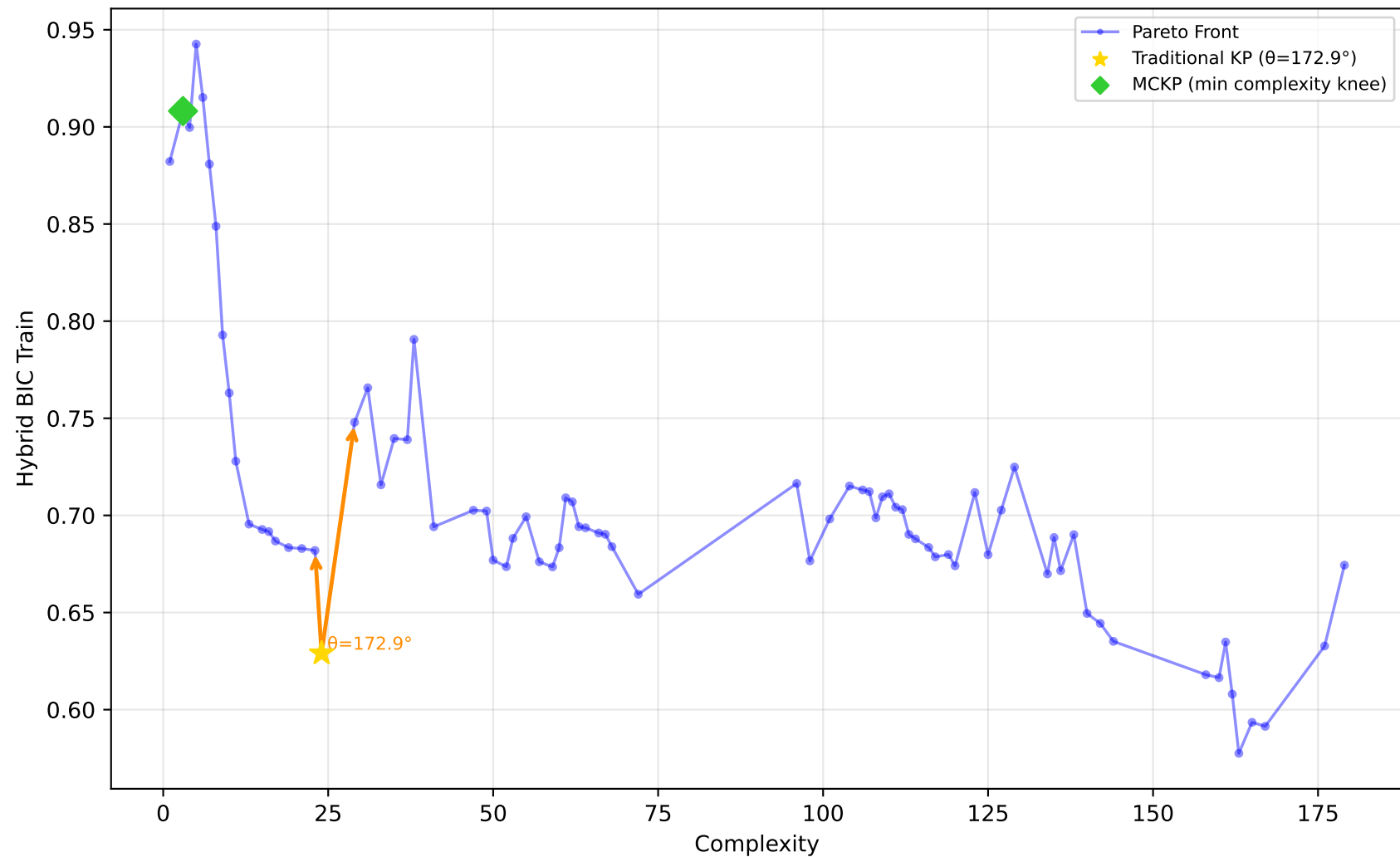
542_pollution - Run 29 - MVP - Hybrid BIC Train \lambda_1=0.40, \lambda_2=0.10, \lambda_3=0.00 | Difficulty: 1.00 | Method: hmr
