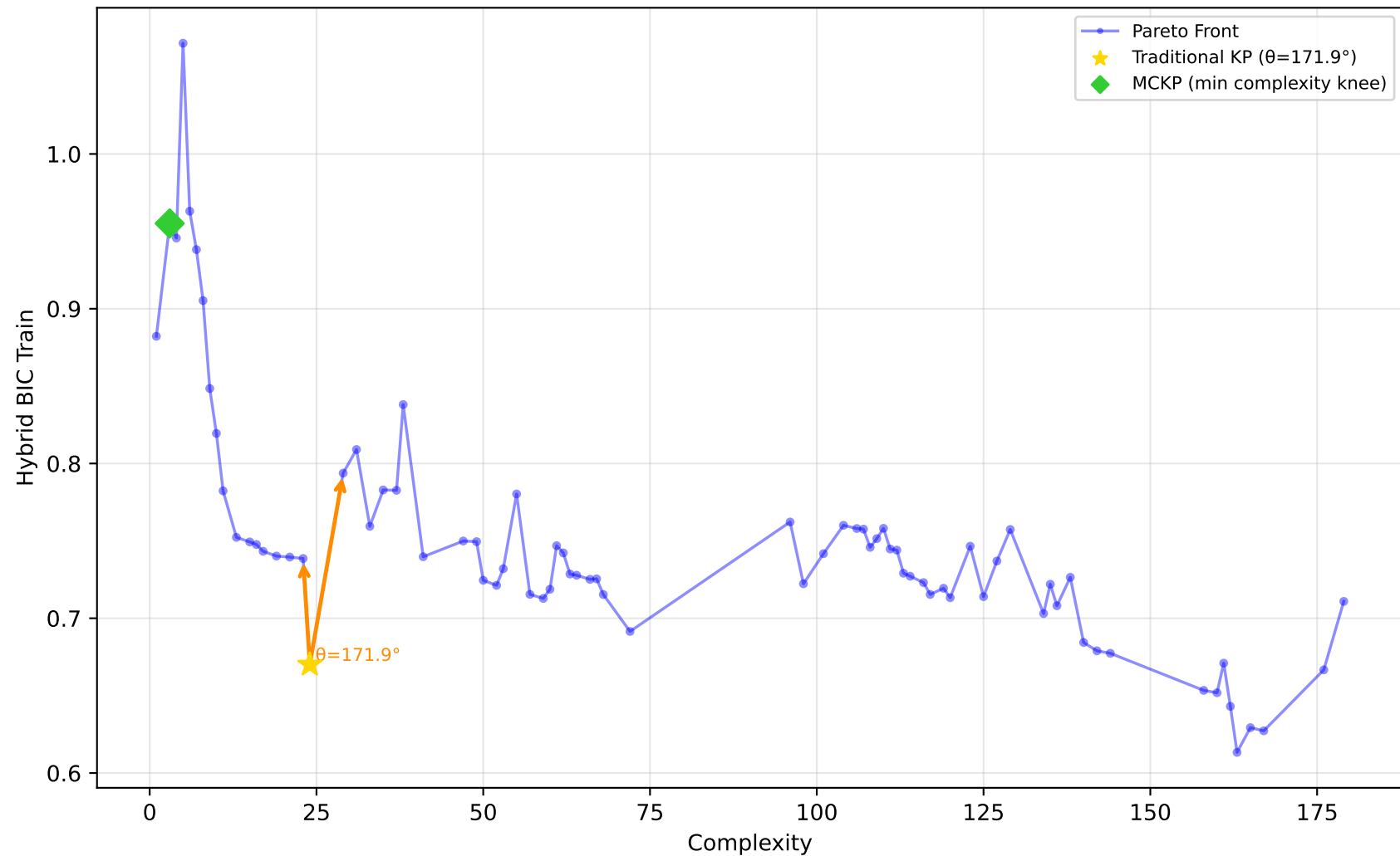
542_pollution - Run 29 - MVP - Hybrid BIC Train \lambda_1=1.00, \lambda_2=0.10, \lambda_3=0.00 | Difficulty: 1.00 | Method: hmr
