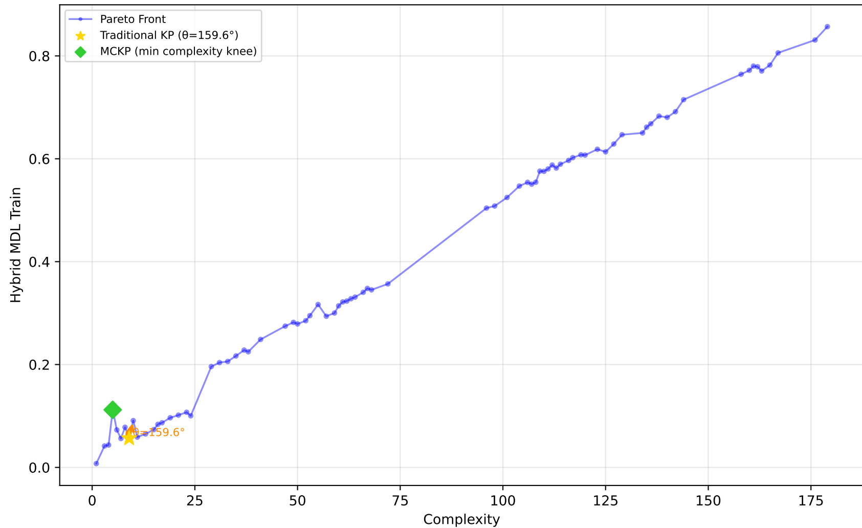
542_pollution - Run 29 - MVP - Hybrid MDL Train \lambda_1=0.40, \lambda_2=0.10, \lambda_3=0.00 | Difficulty: 1.00 | Method: hmr
