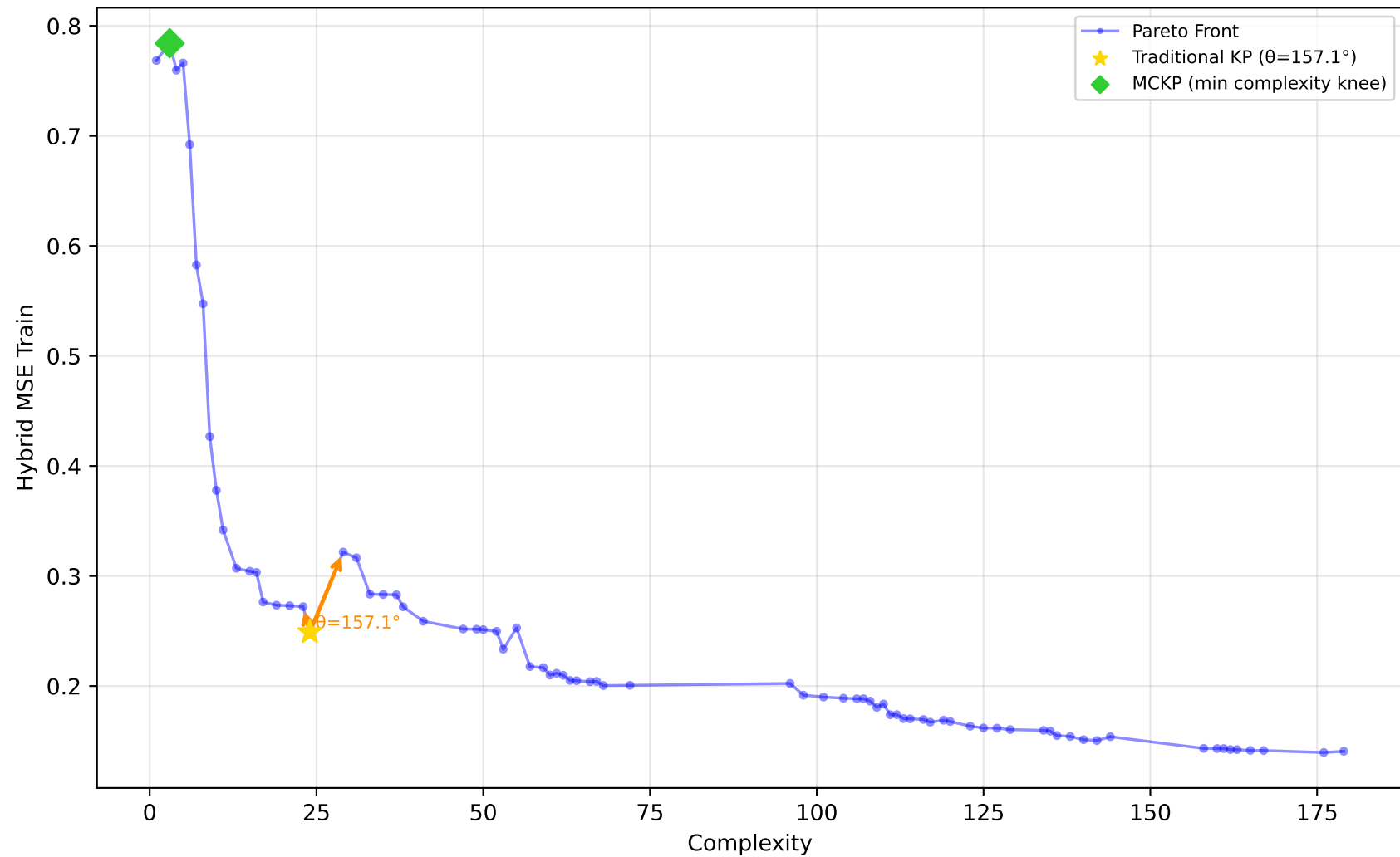
542_pollution - Run 29 - MVP - Hybrid MSE Train \lambda_1=0.40, \lambda_2=0.10, \lambda_3=0.00 | Difficulty: 1.00 | Method: hmr
