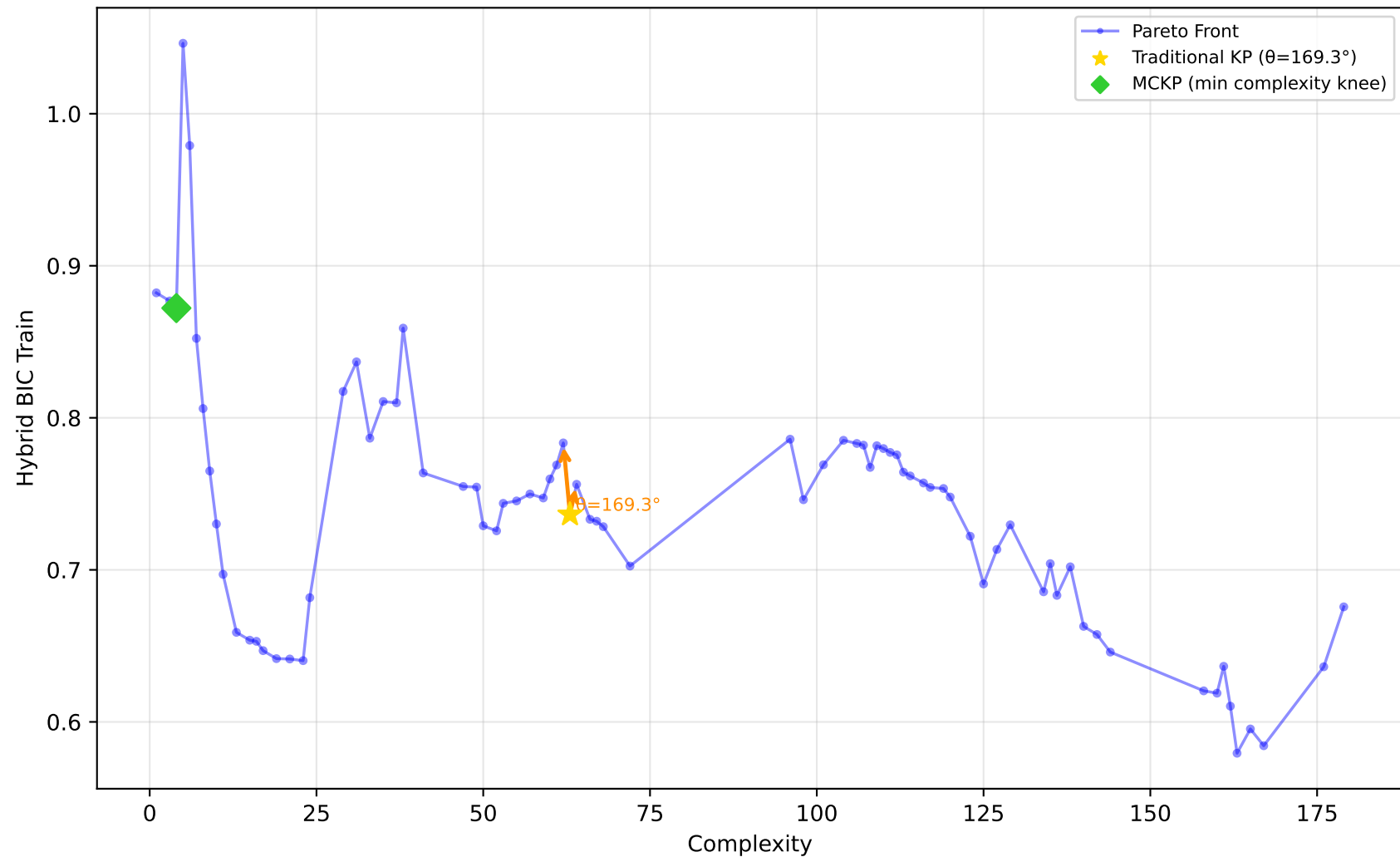
542_pollution - Run 29 - SVP - Hybrid BIC Train \lambda_1=0.00, \lambda_2=0.00, \lambda_3=0.20 | Difficulty: 1.00 | Method: hmr
