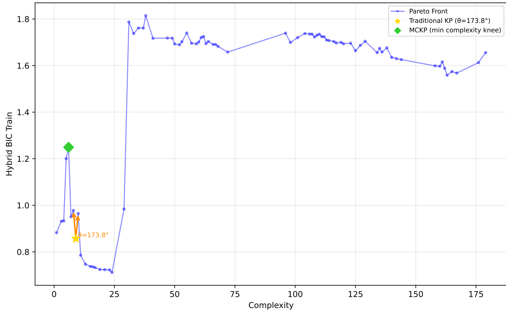
542_pollution - Run 29 - SVP - Hybrid BIC Train \lambda_1=0.70, \lambda_2=1.00, \lambda_3=0.10 | Difficulty: 1.00 | Method: hmr
